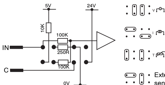
Analogue Input (8 identical channels)
