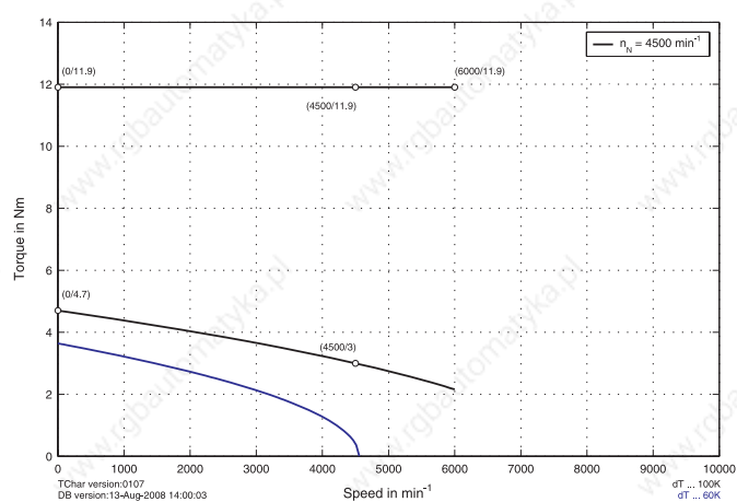
ACOPOSmulti
