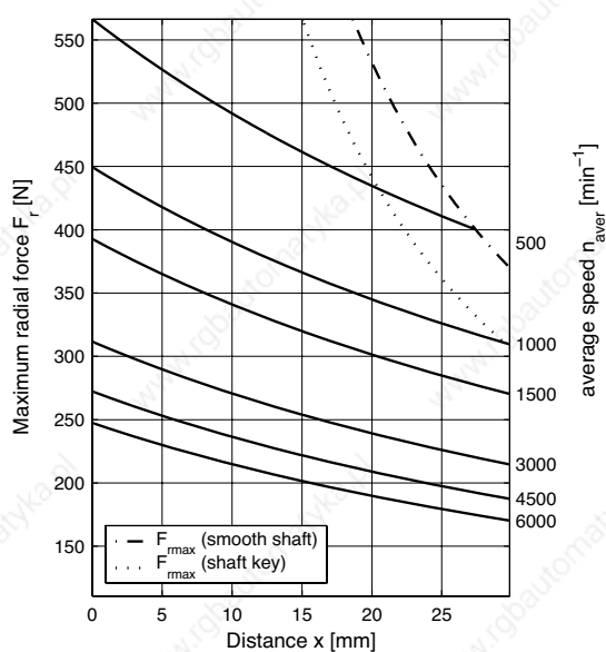
Standard bearing
