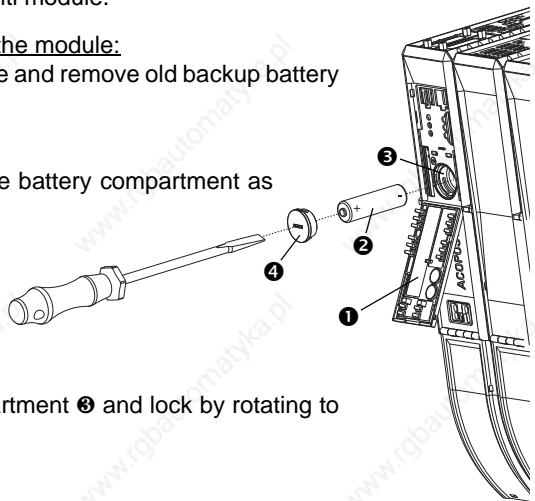
Figure 11: Changing/inserting the backup battery
