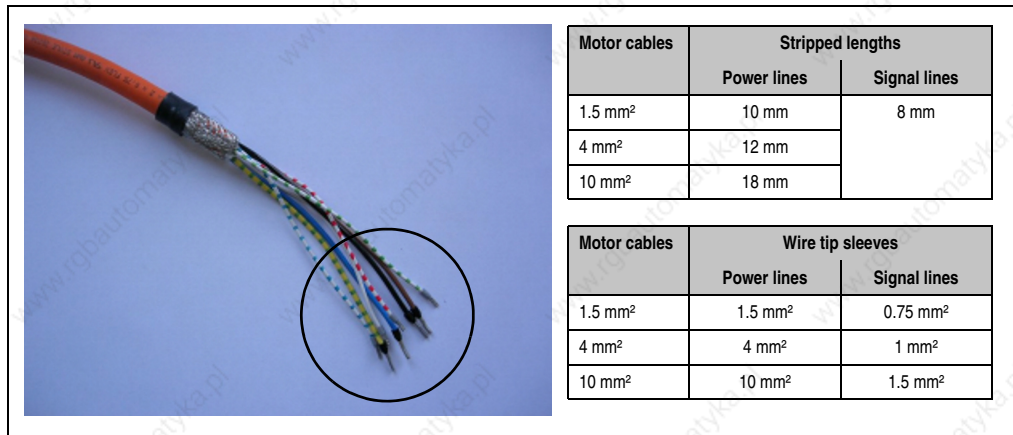
Figure 25: Wire ends with wire tip sleeves
