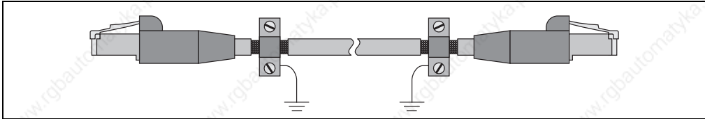
Figure 112: Grounding the POWERLINK cable shielding
