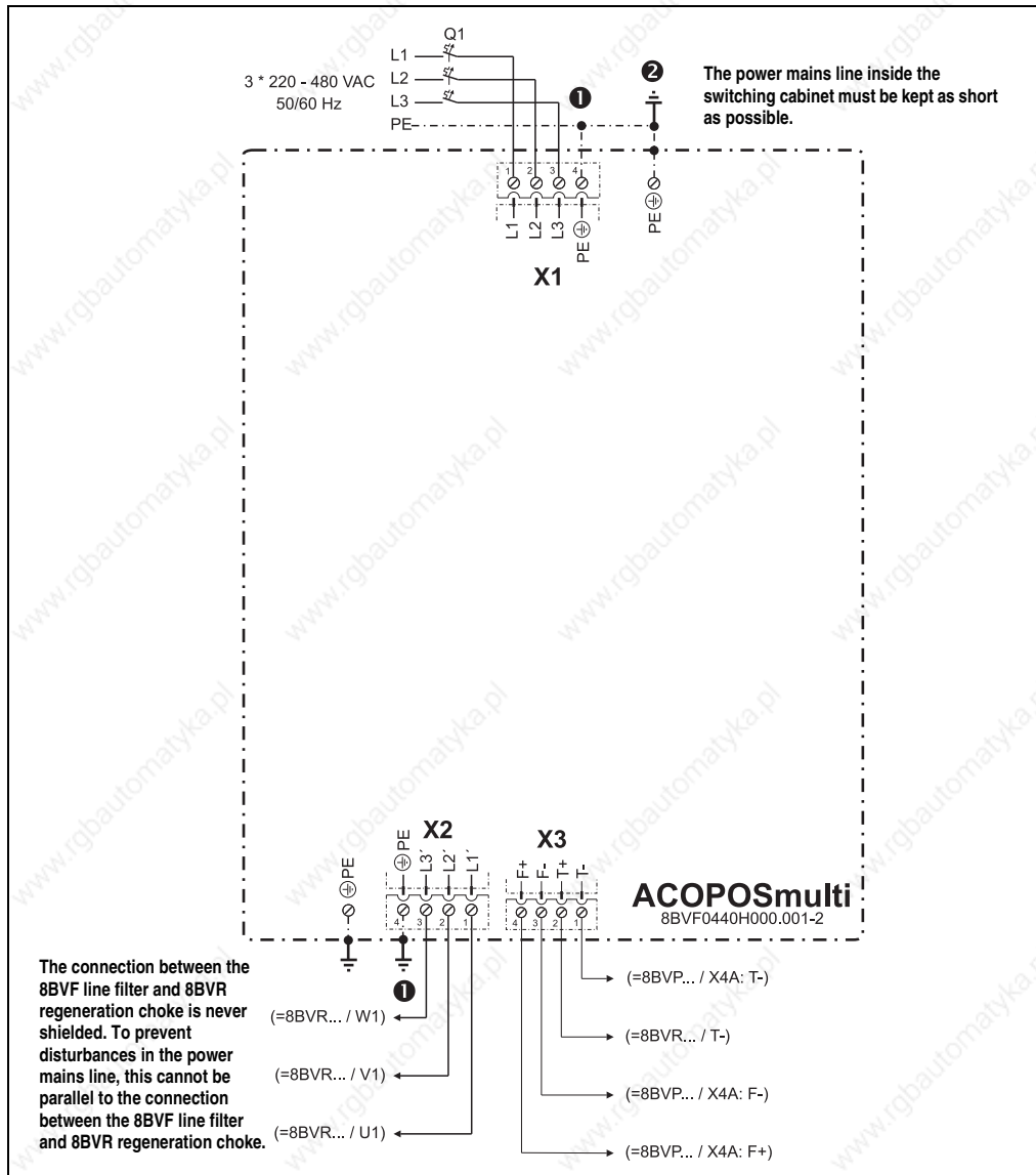
Figure 104: Ground connections and shield connections for 8BVF line filter
