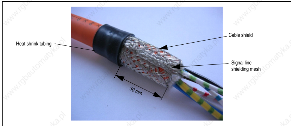
Figure 24: Attaching the shielding mesh
