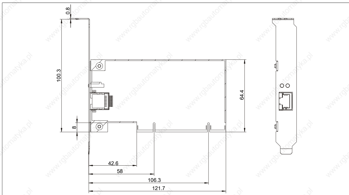
Figure 202: 5ACPCI.ETH1-01 - Dimensions
