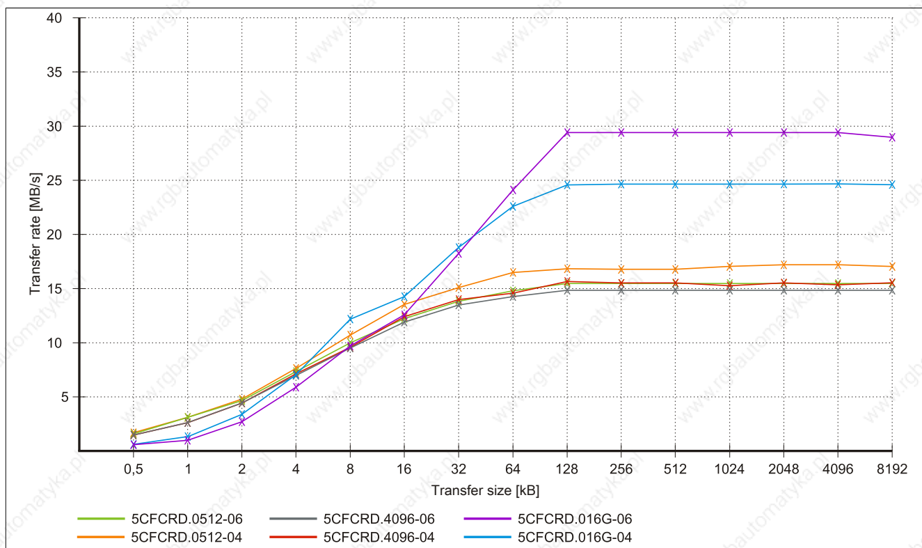
Figure 170: ATTO Disk Benchmark v2.34 write comparison - 5CFCRD.xxxx-04 and 5CFCRD.xxxx-06
