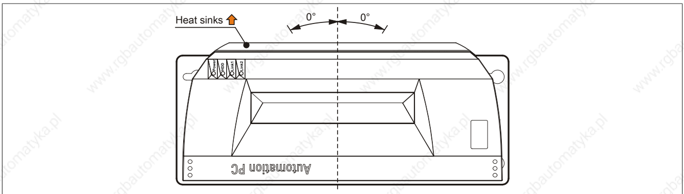
Figure 84: Horizontal mounting orientation
