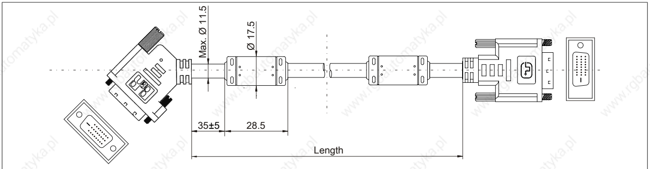
Figure 212: 5CASDL.0xxx-01 - Dimensions
