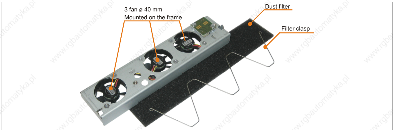
Figure 70: 5PC810.FA01-00 - Fan kit
