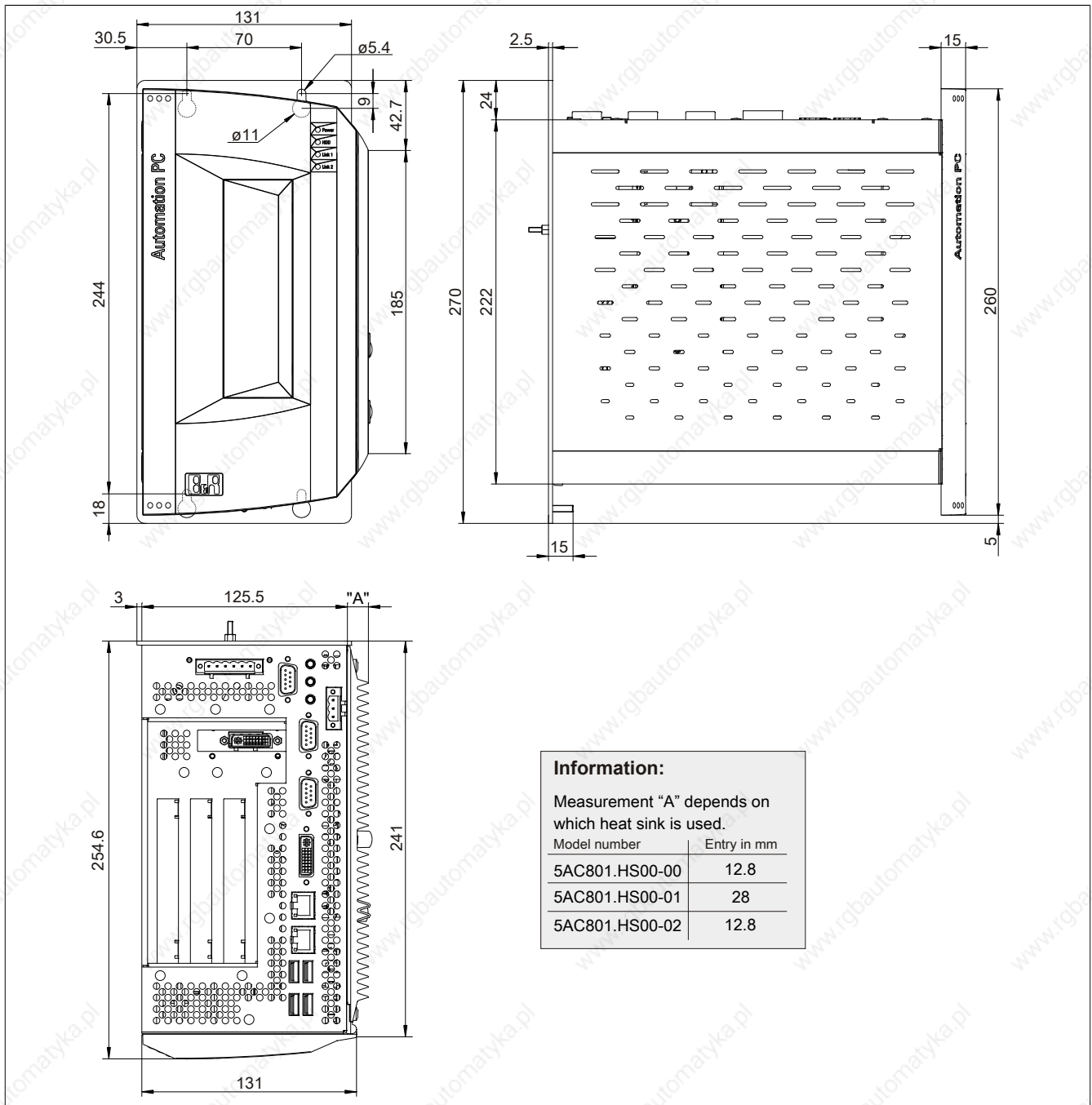
Figure 29: 5PC810.SX03-00 - Dimensions
