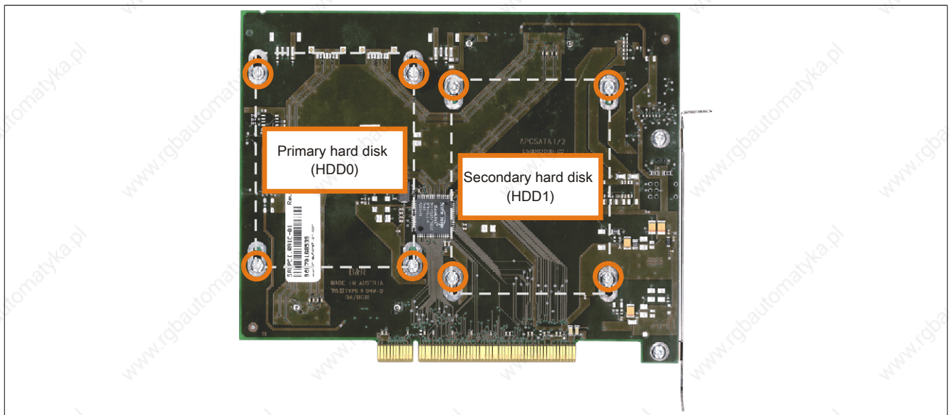
Figure 283: Screw layout on the back side of the 5ACPCI.RAIC-03 SATA RAID controller
