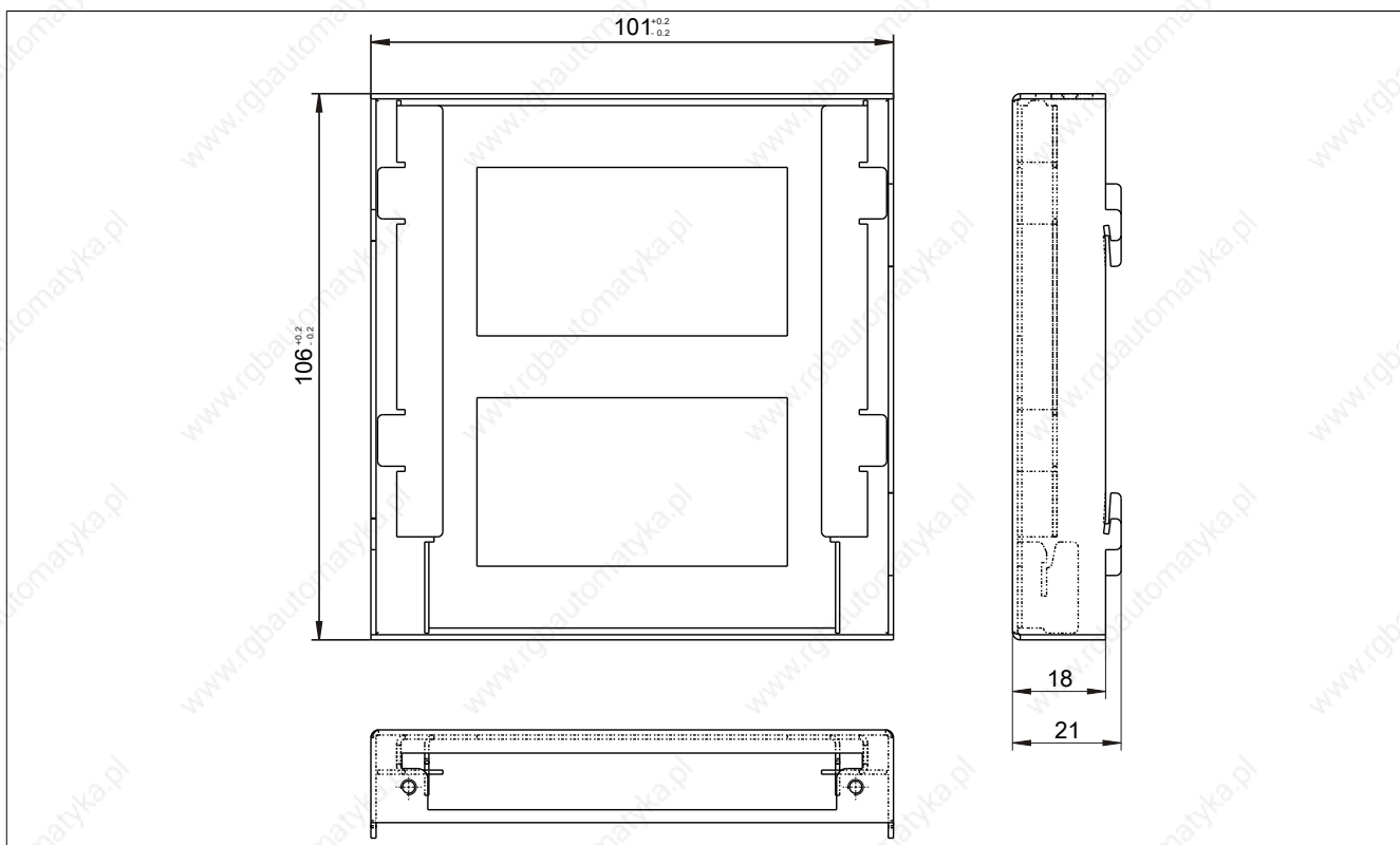
Figure 224: 5AC801.FRAM-00 - Dimensions
