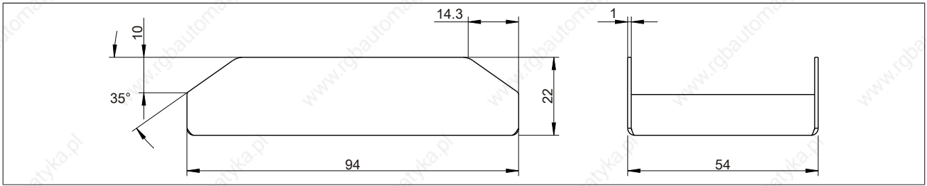
Figure 198: 5AC804.MFLT-00 - Dimensions
