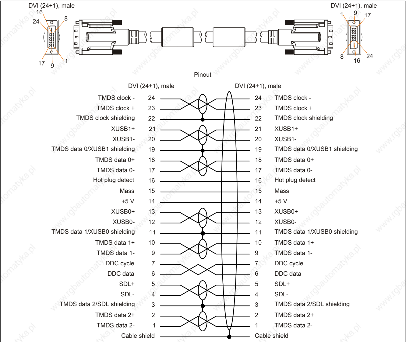
Figure 216: 5CASDL.0xxx-03 - Pinout
