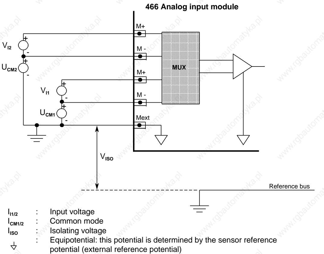
Figure 10-21. Connecting Transducers to the 466 Analog Input Module (Differential Measurement)
