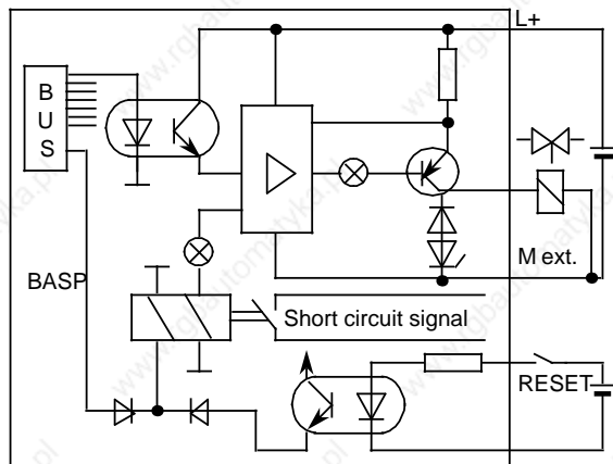
Block diagram
