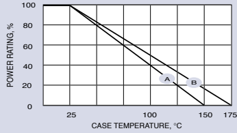
Derating Curve
