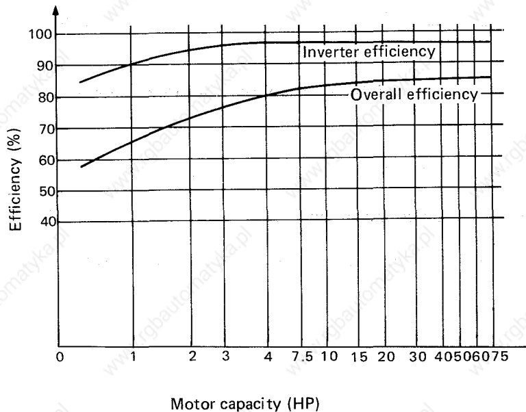
Fig. 12.1 Inverter Efficiency
