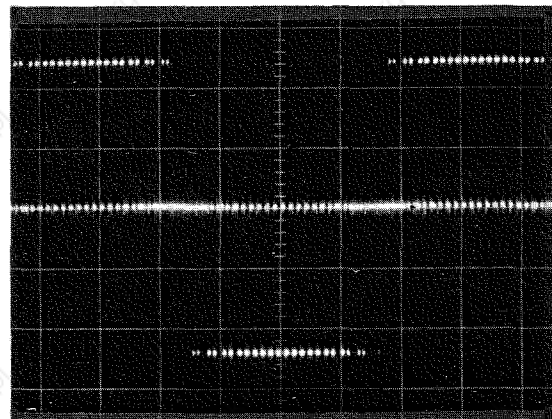
30Hz drive DU-DV, DV-DW or DW-DU 2V/div. 2m sec./div.
