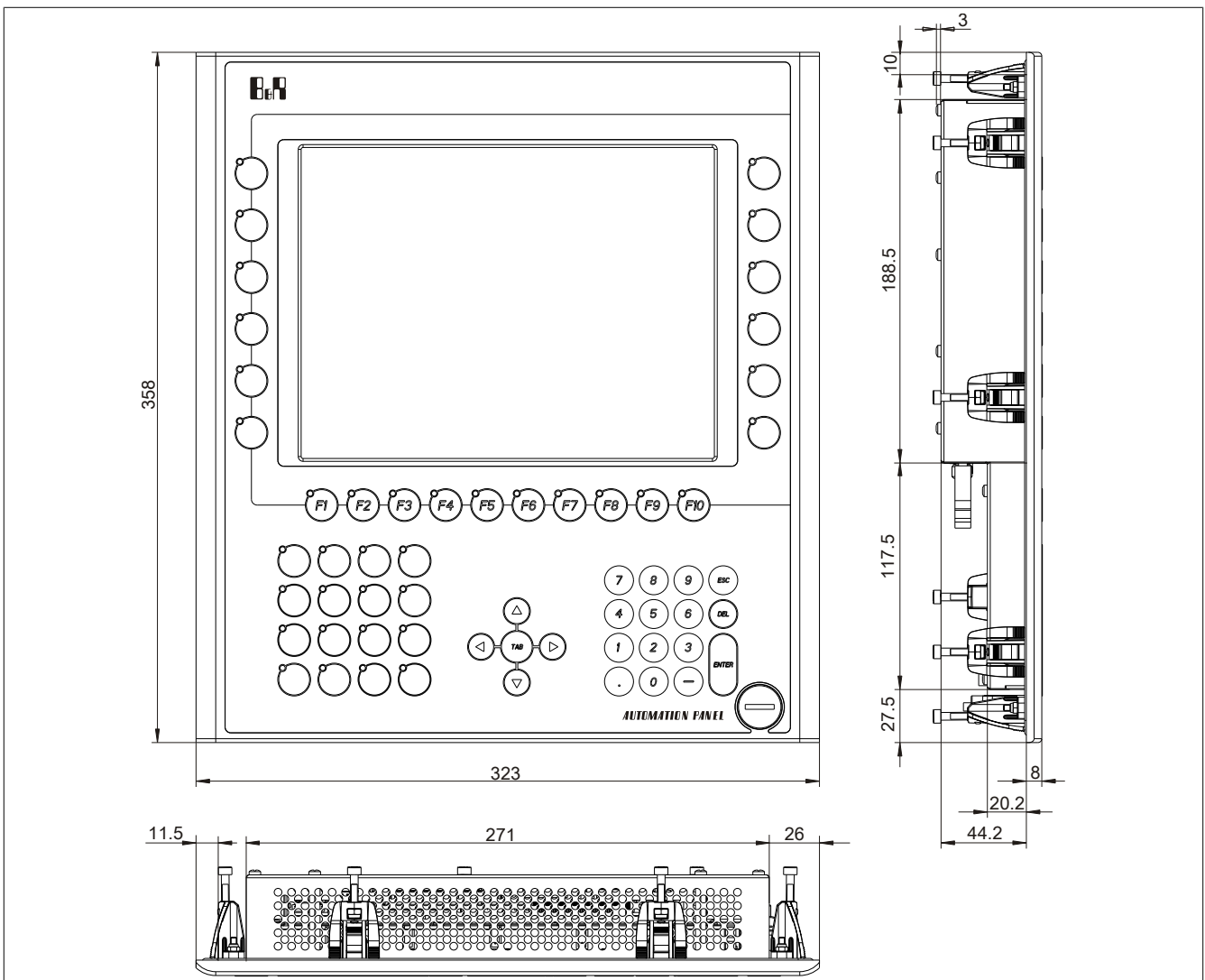
Figure 33: 5AP981.1043-01 - Dimensions
