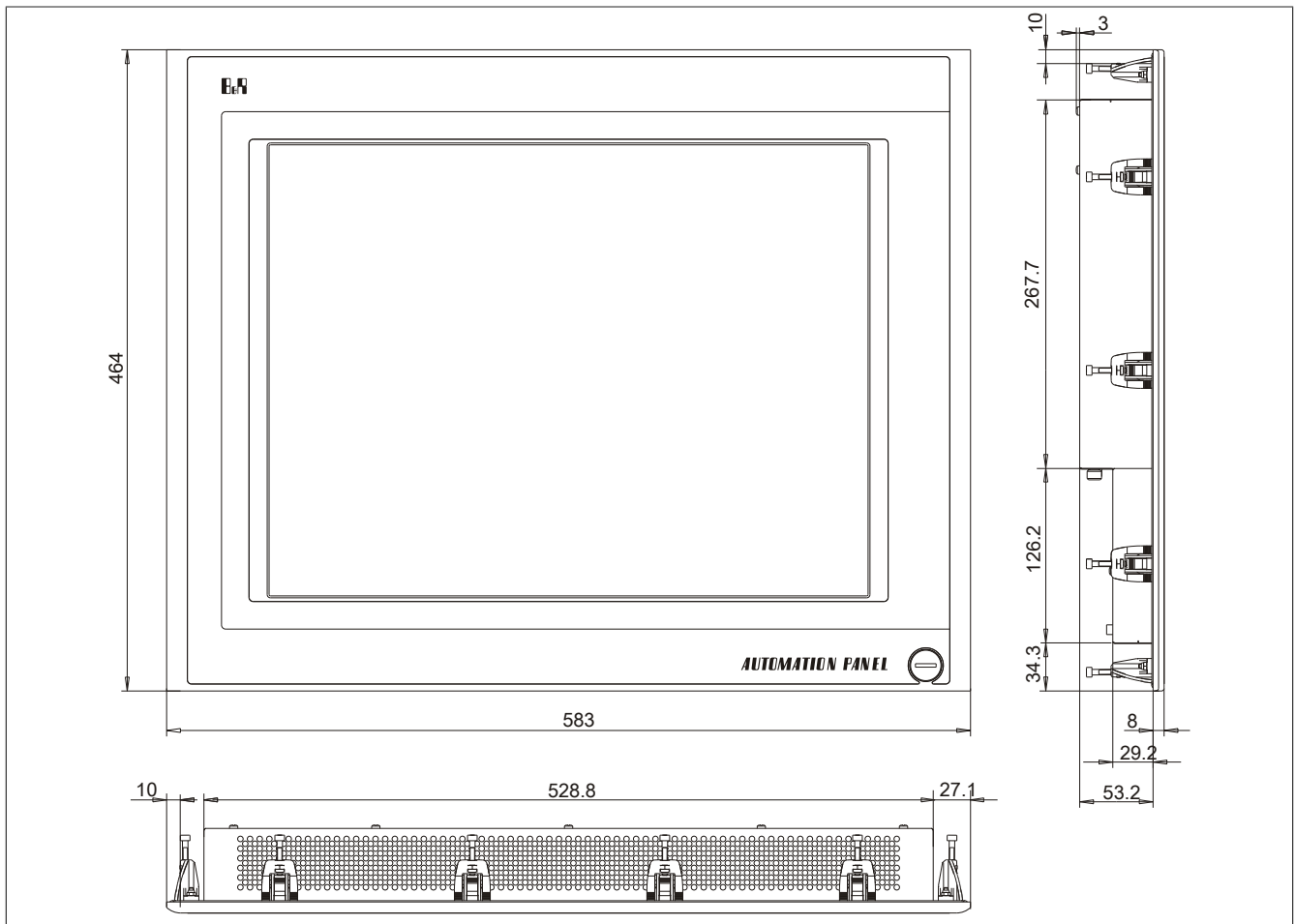
Figure 78: 5AP920.2138-01 - Dimensions
