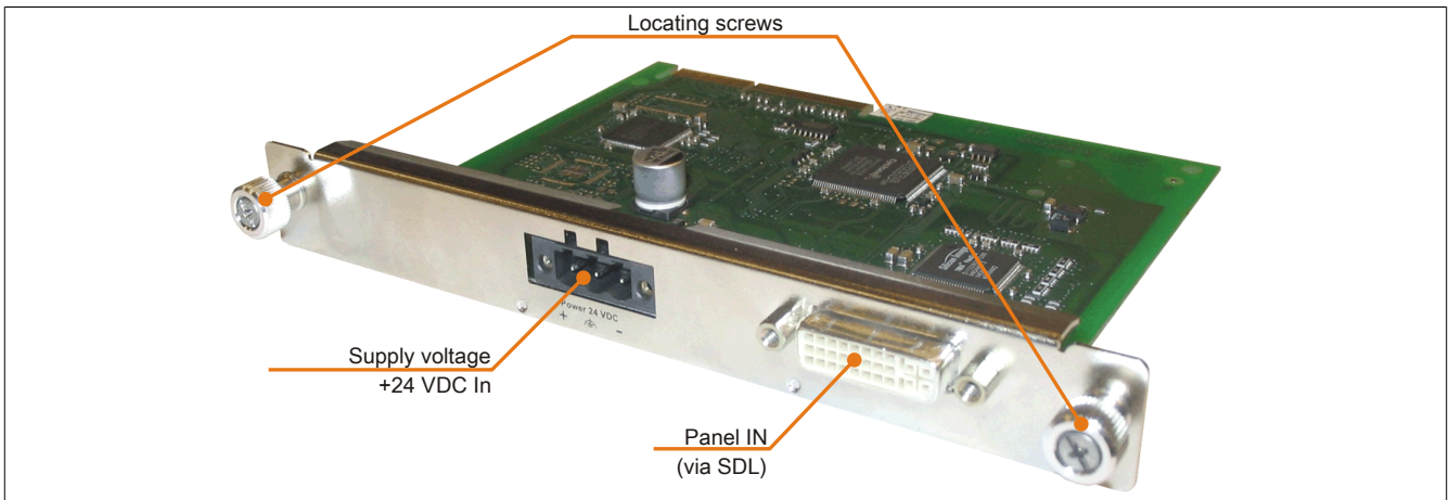
Figure 83: 5DLSDL.1000-00 - Interfaces
