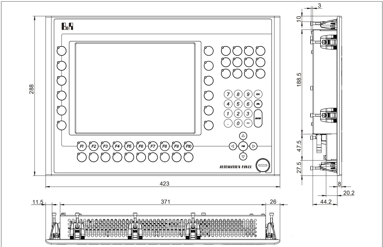
Figure 23: 5AP952.1043-01 - Dimensions
