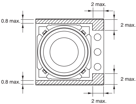
Supporting and Mounting Area (Shaded Portion) Top View
