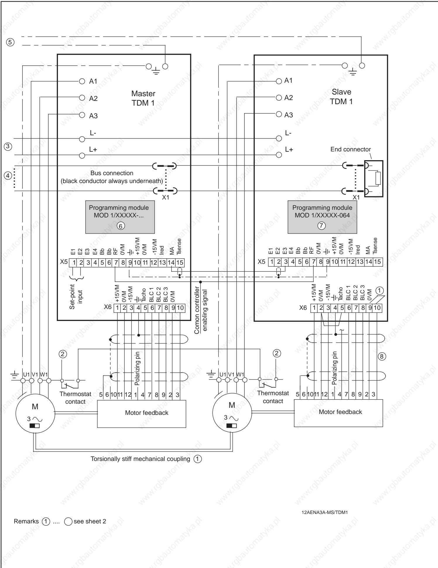
Fig. 12: Connection diagram for master-slave drive with TDM 1
