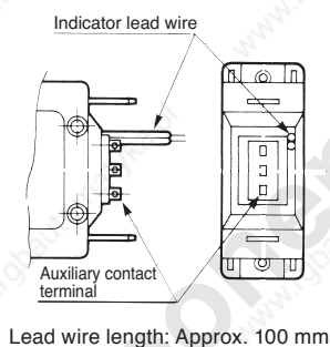
Illuminated Rocker Type (1-pole) Relay Trip (4-terminal)
