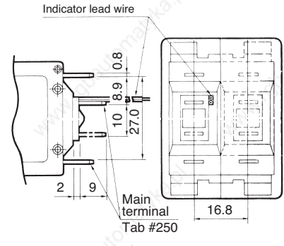
Illuminated Rocker Type (2-pole) Relay Trip (4-terminal)
