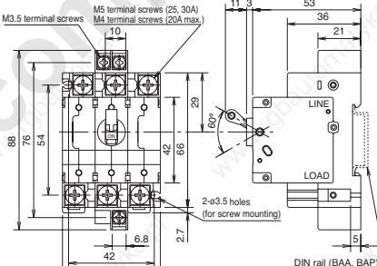
Series Trip (Auxiliary/Alarm Contacts)
