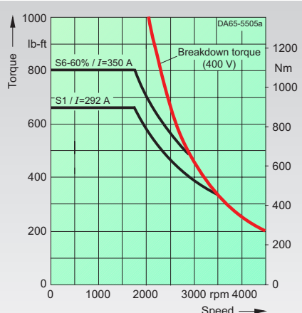
1PL6224-4.F. max. breakdown torque: 1257 lb-ft/1704 Nm
