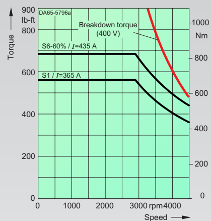
1PL6224-4.L. max. breakdown torque: 1125 lb-ft/1526 Nm
