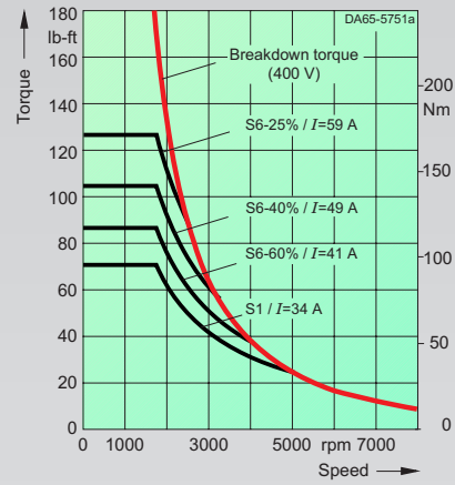
1PH7133-2.F.-..... max. breakdown torque: 184 lb-ft/250 Nm
