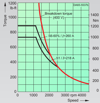
1PL6224-4.D. max. breakdown torque: 1532 lb-ft/2077 Nm
