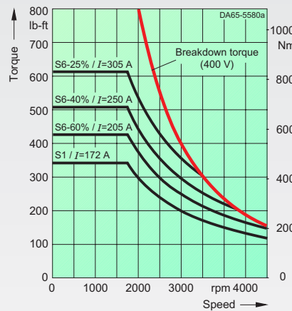
1PH7186-2.F.-..... max. breakdown torque: 1014 lb-ft/1375 Nm
