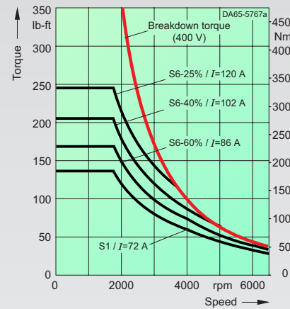
1PH7163-2.F.-..... max. breakdown torque: 512 lb-ft/694 Nm
