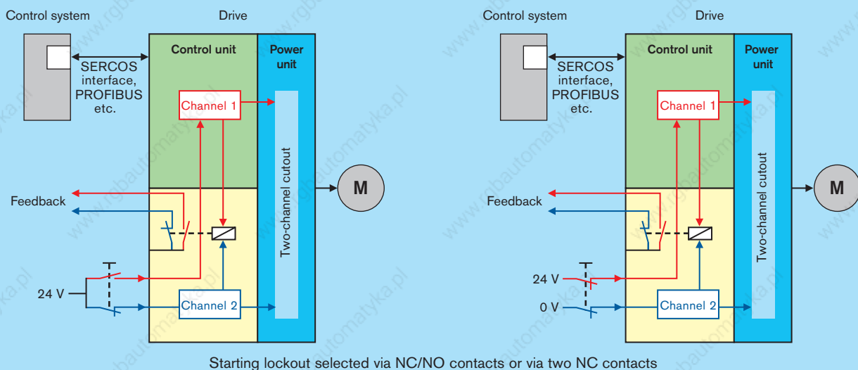
Starting lockout selected via NC/NO contacts or via two NC contacts
