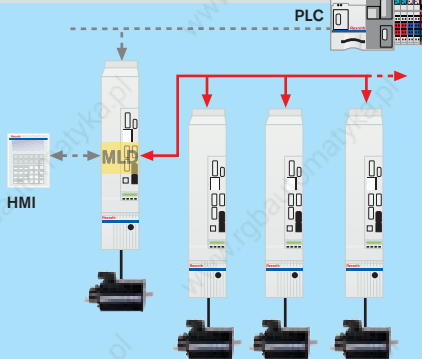
IndraMotion MLD-M Integrated Motion Logic with cross communication
