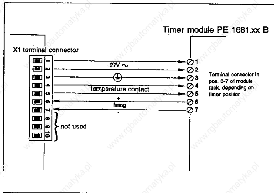
Fig. 5.9 Pin assignment
