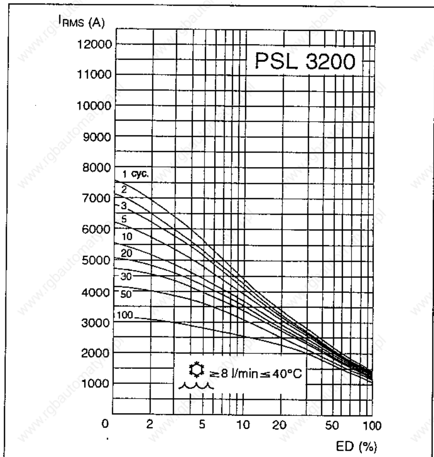
Fig. 3.3 Load diagram
