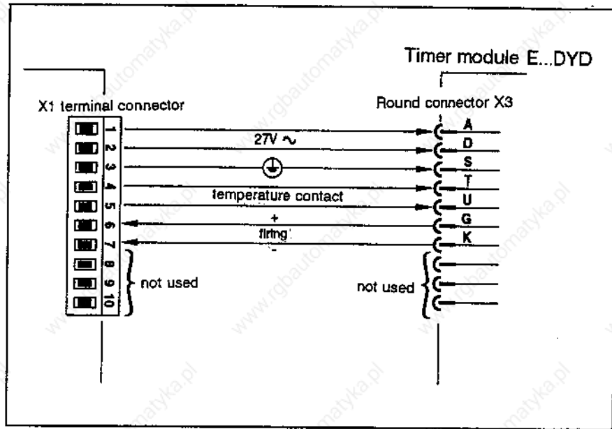
Fig. 5.8 Pin assignment
