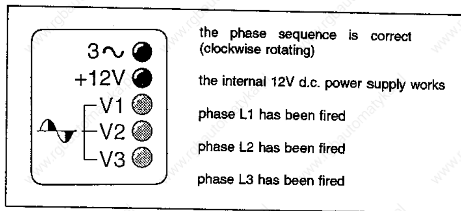
Fig. 8.1 LED display
