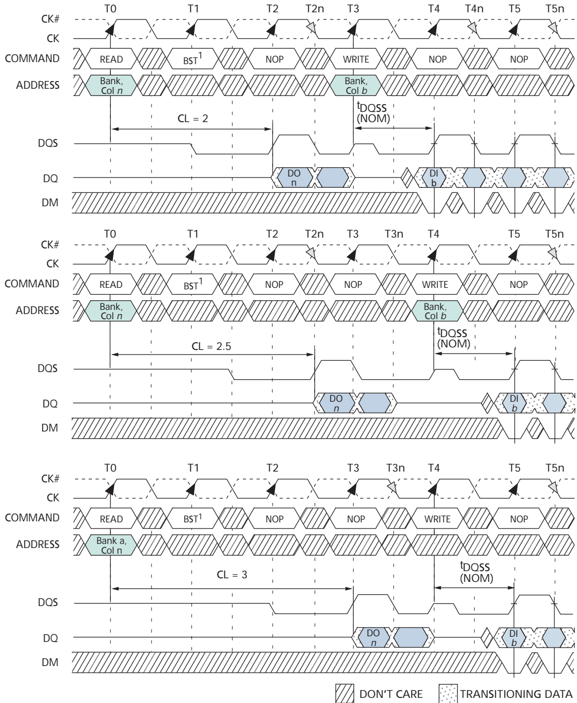
Figure 32: READ-to-WRITE
