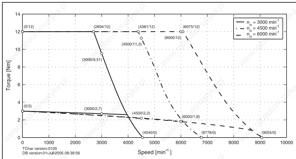
Figure 18: Speed - torque characteristic curve for 8LSA36.eennnffgg-0
