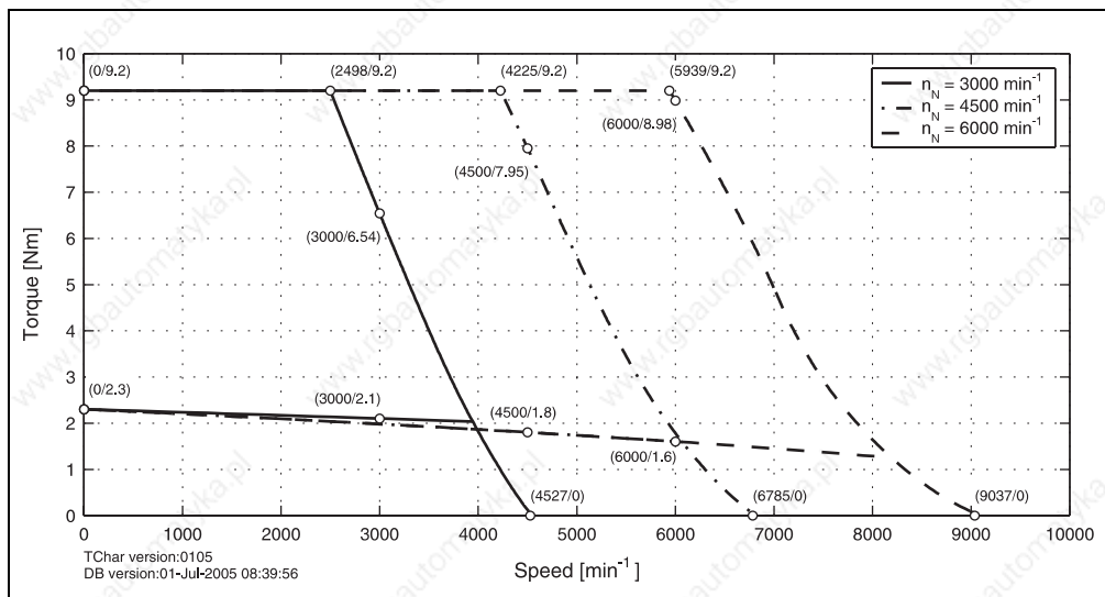
Figure 17: Speed - torque characteristic curve for 8LSA35.eennnffgg-0
