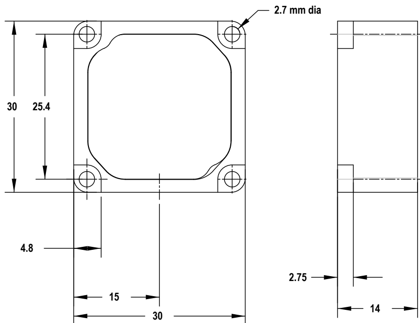
Figure 2. Stainless steel models
