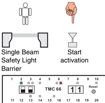
Fig. 5.12-1: Waiting mode
