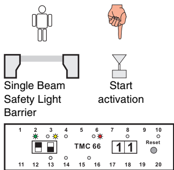
Fig. 5.13-1: Waiting mode
