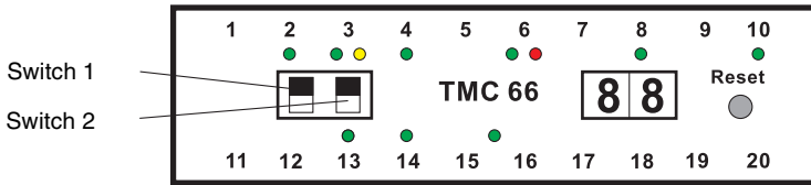
Fig. 5.10-3: Adjustment of the operating mode (start- and restart interlock active, contactor monitoring active)
