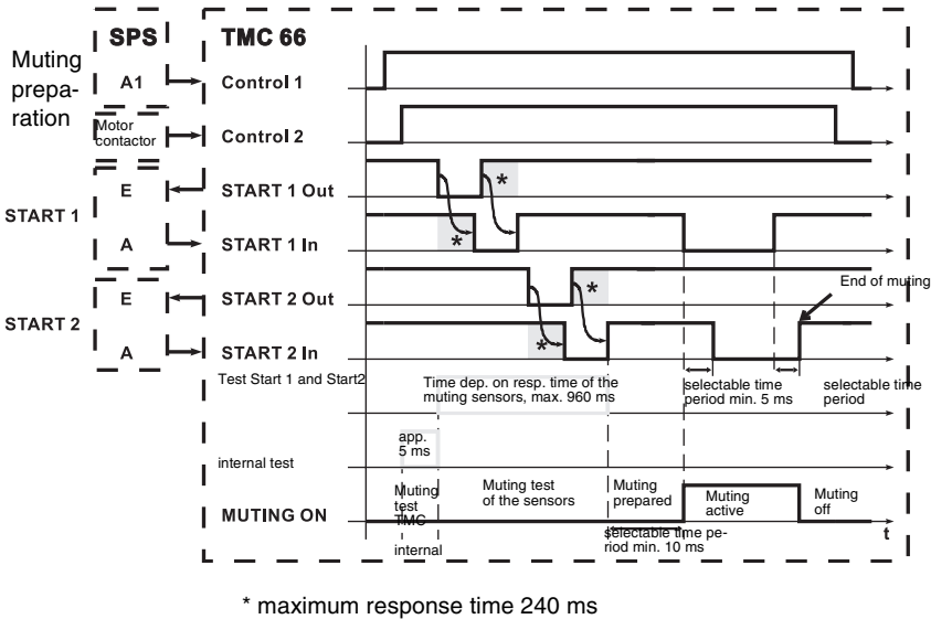
Fig. 4.2-6: Signal flows during muting
