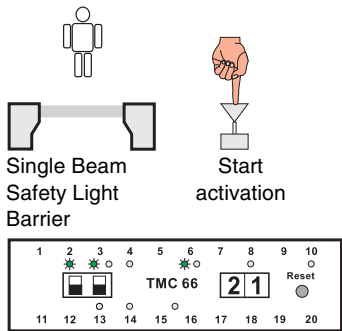
Fig. 5.12-2: Protection mode
