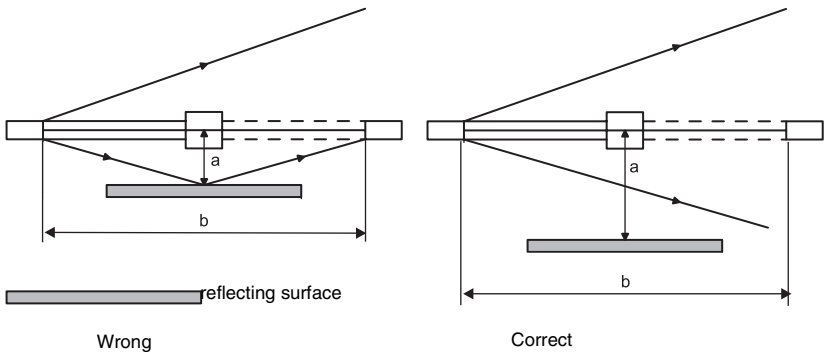
Fig. 4.2-4: Reflection bypass
