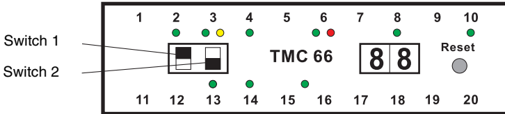
Fig. 5.10-1: Adjustment of the operating mode (start- and restart interlock active, contactor monitoring inactive)
