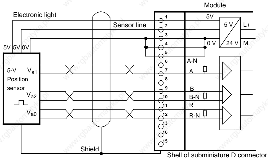
Figure 15-11. Connecting a 5-V Position Sensor to RS 422
