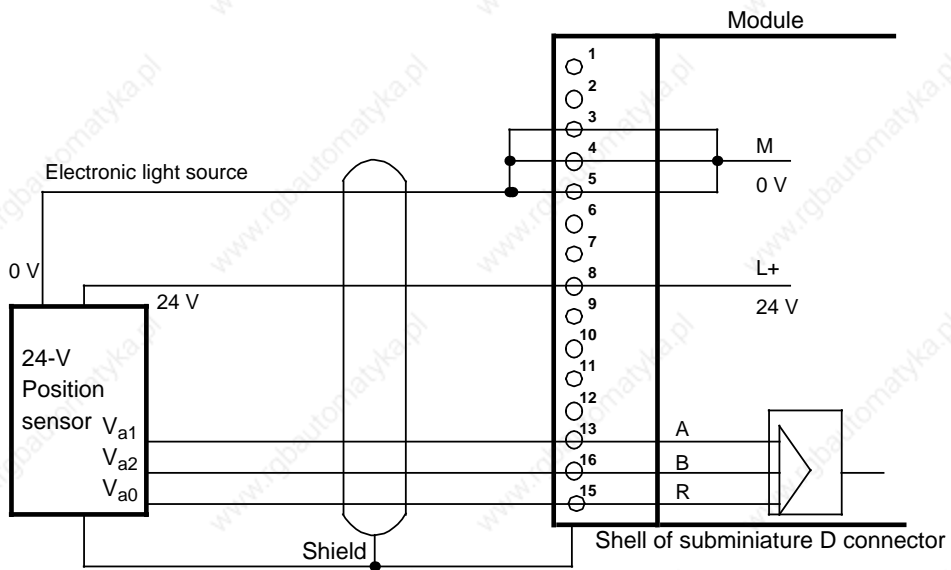
Figure 15-12. Connecting a 24 V DC Position Sensor
