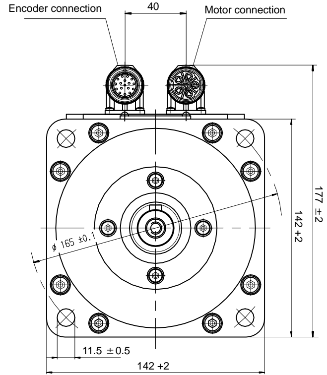
Motor type SF(R)-B4.0091/0125.060
