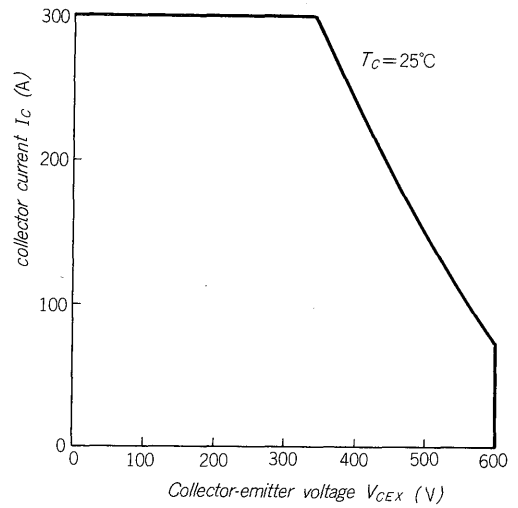
Fig. 19 RBSOA of EVK71-050A at overcurrent
