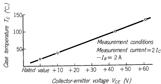
Fig. 10 RBSOA- T_j characteristics of EVK71-050A
