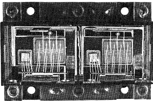
Fig. 2 Interior structure of power transistor module
