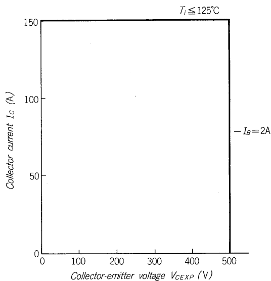
Fig. 9 Reverse biased SOA of EVK71-050A
