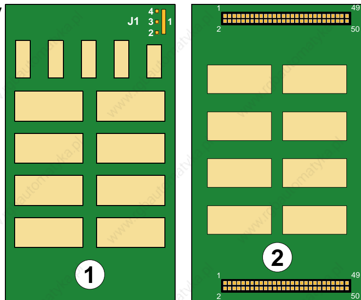
Figure A-1: DM600 Memory Piggyback
