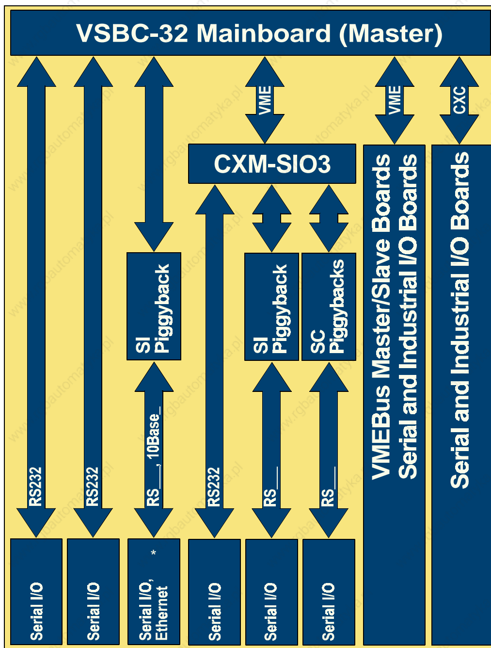
Figure 1-1: VSBC-32(E) System-Level Functional Block Diagram
