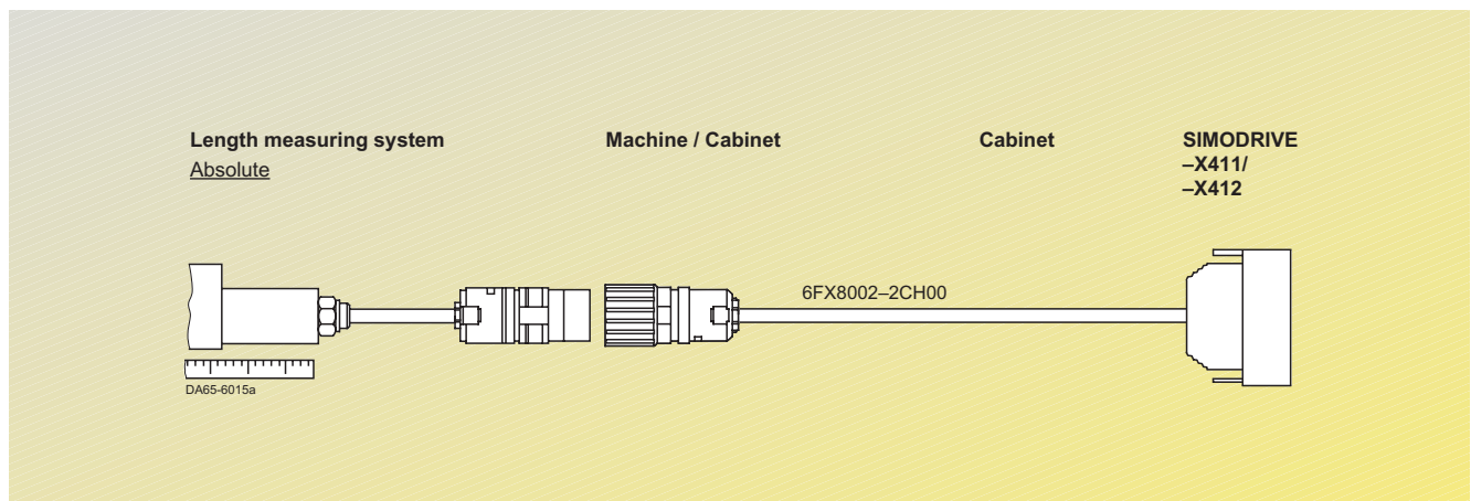
Fig. 5/2 Termination technology for absolute-value measuring system on 1FN3 motors
