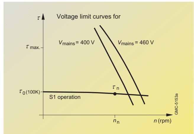
Fig. 2/2 Torque-speed characteristic
