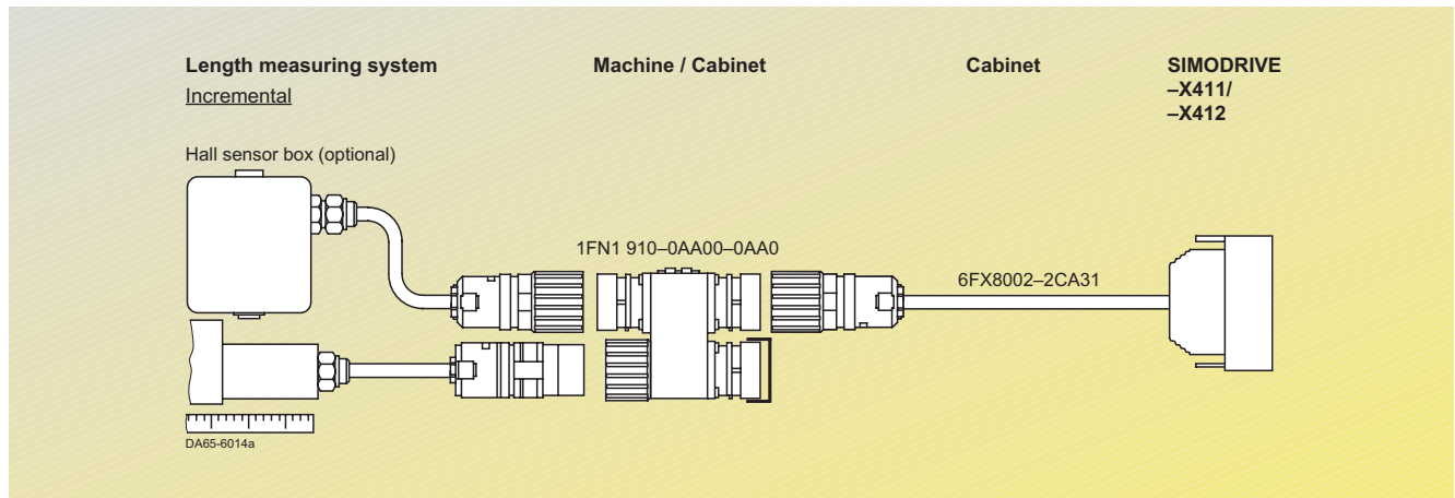
Fig. 5/1 Termination technology for incremental measuring system on 1FN3 motors
