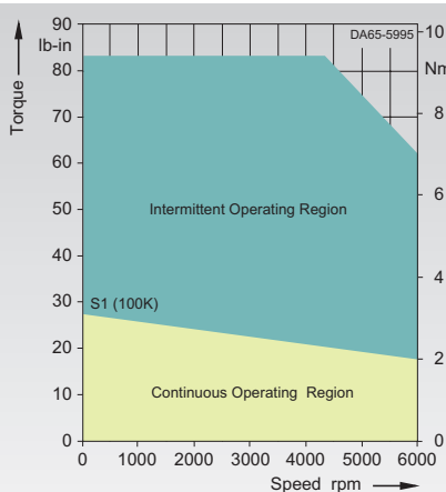
1FK6043-7AK71-1...
