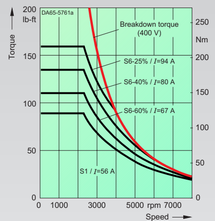
1PH7137-2.G...-.... max. breakdown torque: 276 lb-ft/375 Nm
