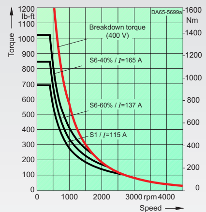
1PH7226-2.B.-..... max. breakdown torque: 1661 lb-ft/2252 Nm
