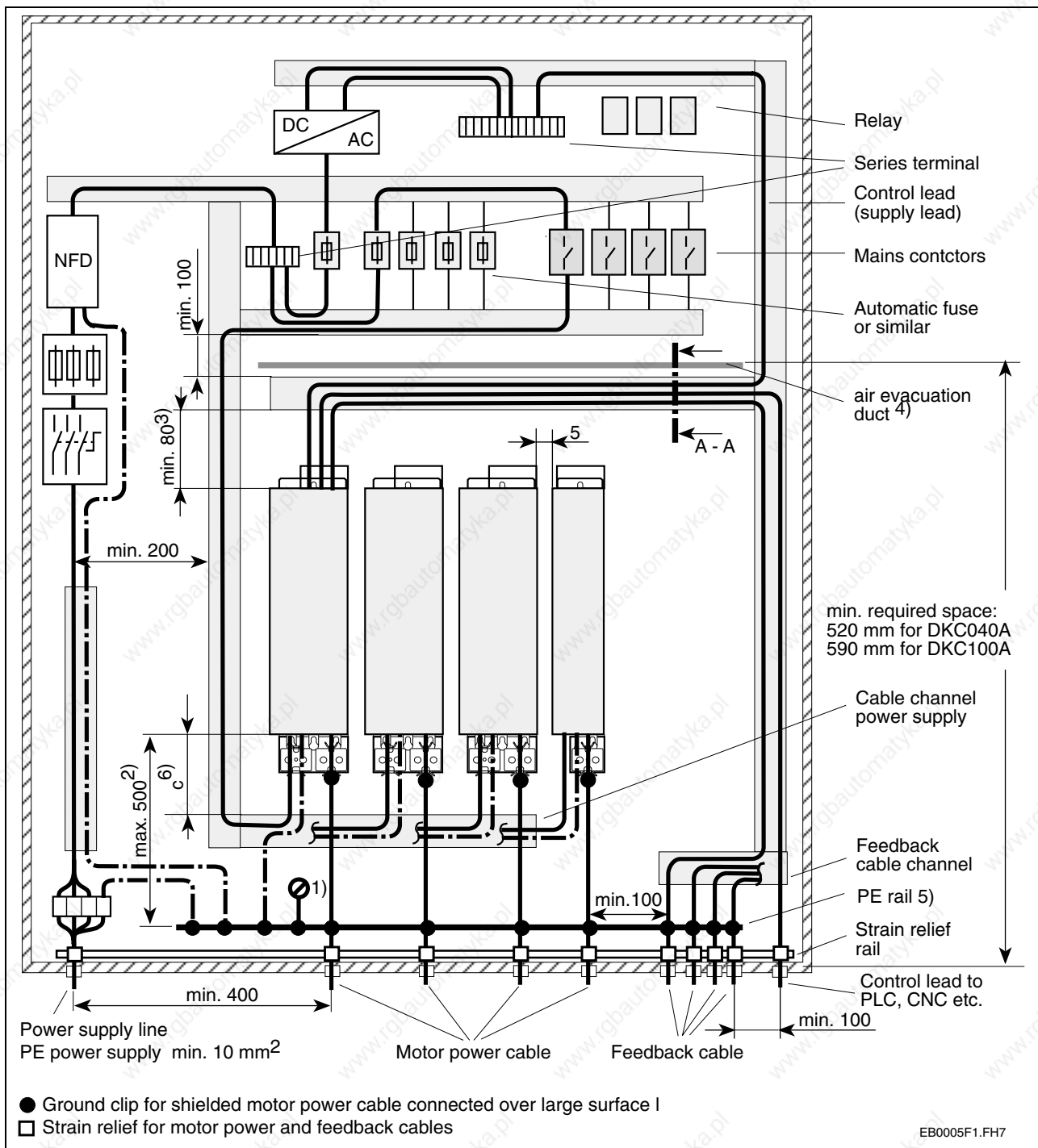
Fig. 16-14: Recommendations on constructing the control cabinet
