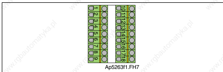
Fig. 4-138: Connector X11
