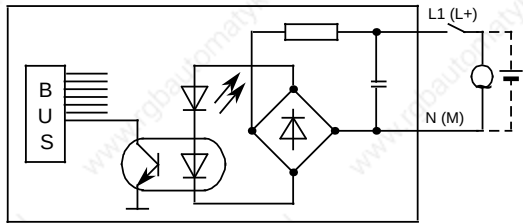
Block diagram
