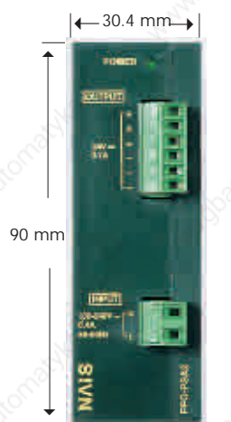
FP0 Power supply FP0-PSA2
