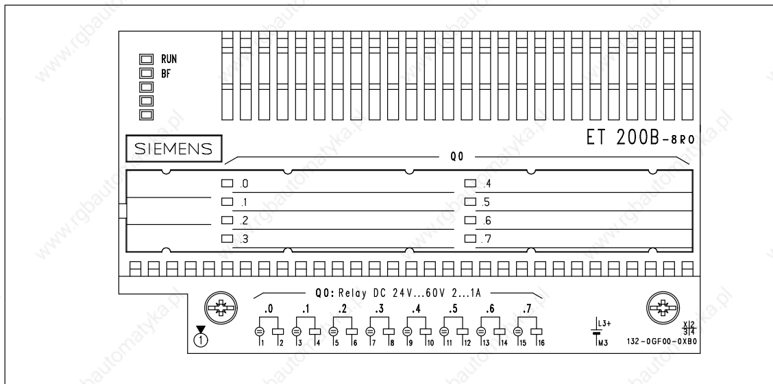
Figure 8-29 Front Elevation: ET 200B-8RO (6ES7 132-0GF00-0XB0)
