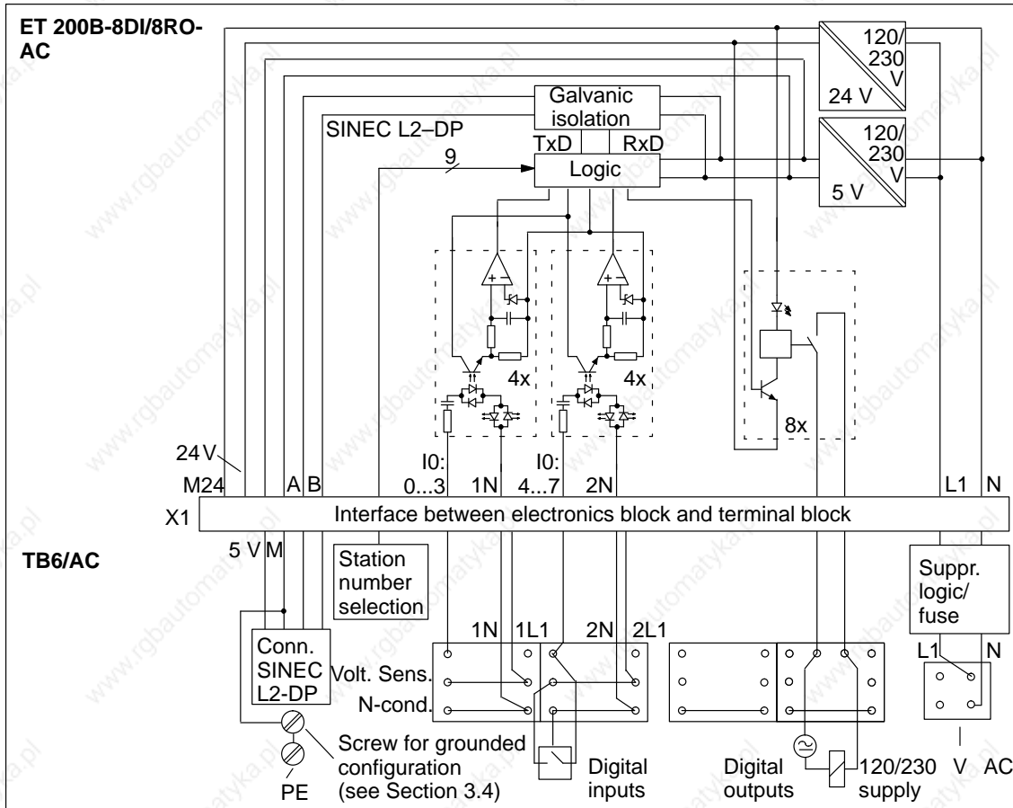
Figure 8-45 Schematic Circuit Diagram: ET 200B-8DI/8RO-AC (6ES7 133-0HH00-0XB0) and TB6/AC
