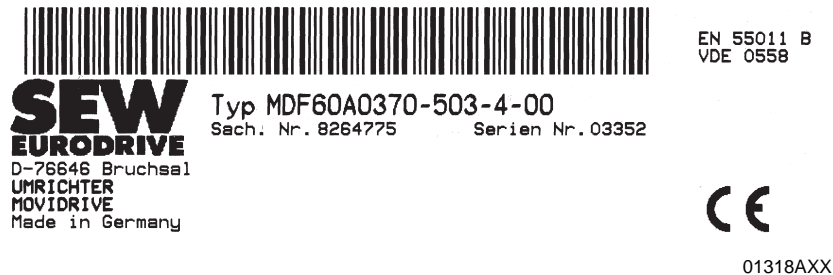
Fig. 2: Overall nameplate
