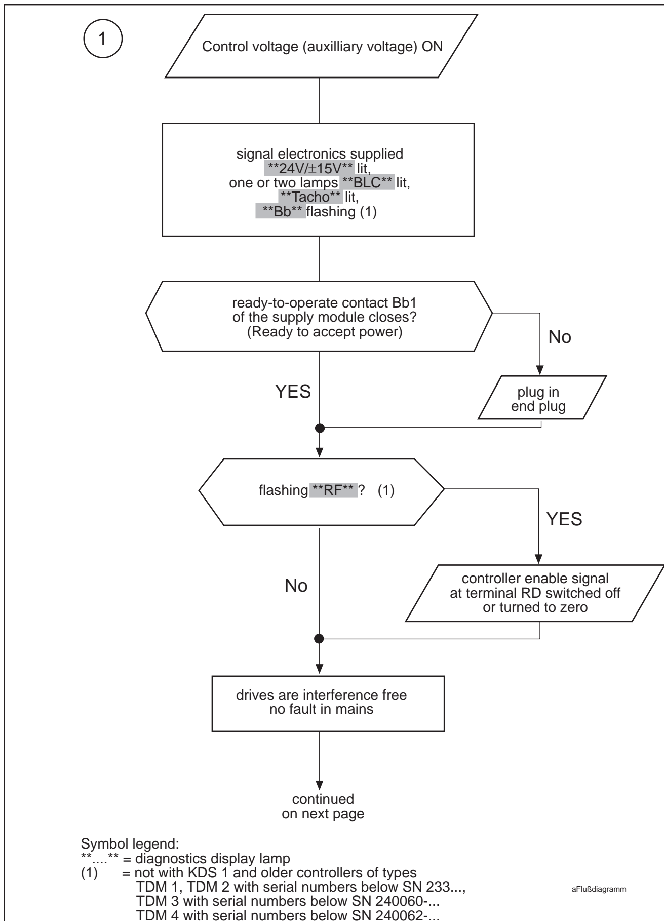
Figure 72: Power-Up Sequence
