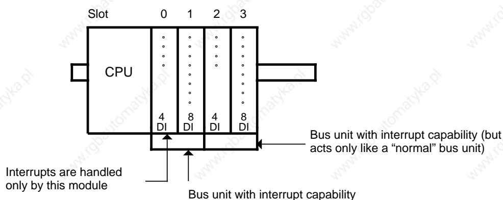
Figure 10-1. Possible Configuration of the Programmable Controller with Bus Units Having Interrupt Capability
