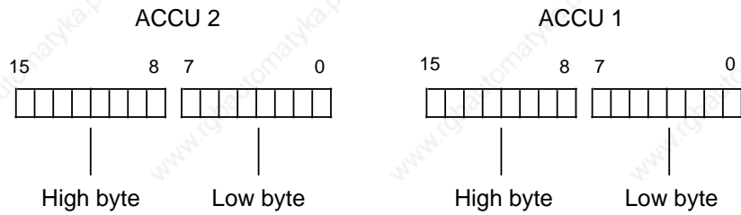
Figure 8-1. Accumulator Structure
