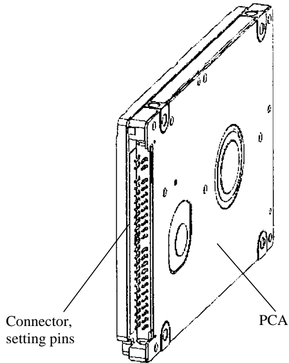
Figure 3.8 Connector locations
