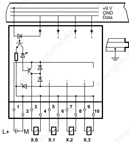
DIGITAL OUTPUT 4 x 24 - 60 V DC/0.5A 6ES5 450-8MB11
