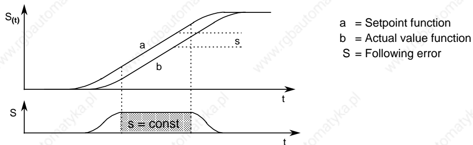
Figure 15-28. Course of a Following Error during a Positioning Operation
