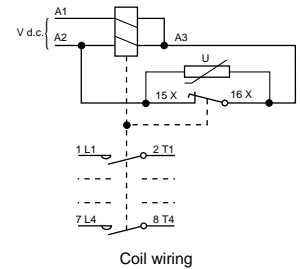
Coil wiring
