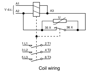
Coil wiring
