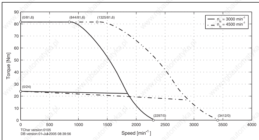
Figure 47: Speed - torque characteristic curve for 8LSA65.eennnffgg-0
