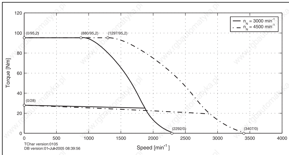
Figure 48: Speed - torque characteristic curve for 8LSA66.eennnffgg-0
