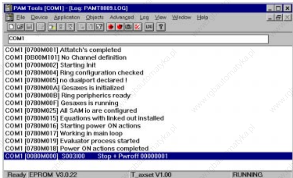
Figure 53 PAM Tools Main Window with Activity Log Displayed
