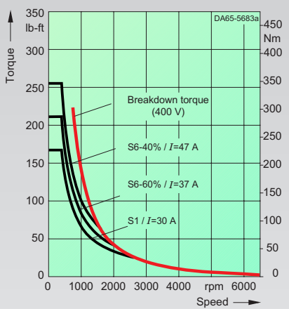
1PH7163-2.B.-..... max. breakdown torque: 458 lb-ft/621 Nm
