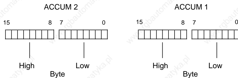
Figure 8-1. Accumulator Structure
