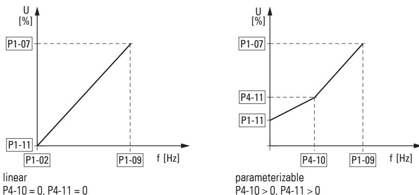
Figure 68: V/f-characteristic curve
