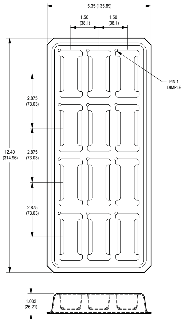
Figure 13. Shipping Tray
