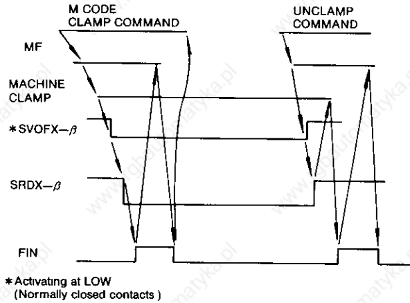
Fig 19 21 Time Chart of Servo Off Signal
