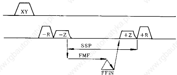
Fig 19 14 Time Chart of G86 through G89
