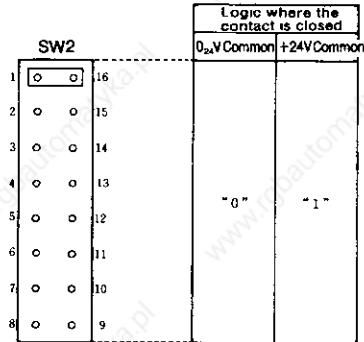
Shorting Plug Setting on SW2 No.1
