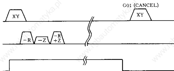
Fig 19 20 Canned Cycle ON Signal (G80S)
