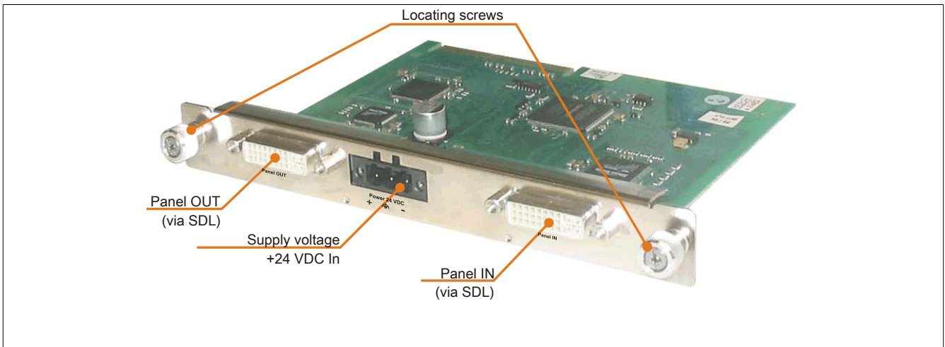
Figure 84: 5DLSDL.1000-01 - Interfaces
