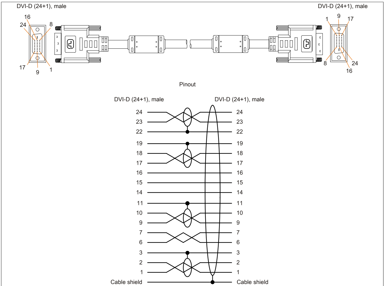
Figure 117: 5CADVI.0xxx-00 - Pinout
