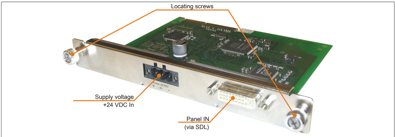
Figure 83: 5DLSDL.1000-00 - Interfaces
