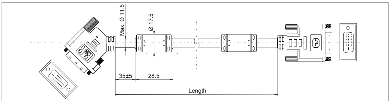
Figure 122: 5CASDL.0xxx-01 - Dimensions
