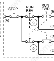
3-WIRE CONTROL
