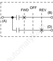
2-WIRE CONTROL W / O AUTO
