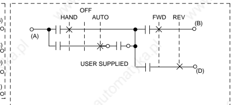
2-WIRE CONTROL W / AUTO START MANUAL DIRECTION
