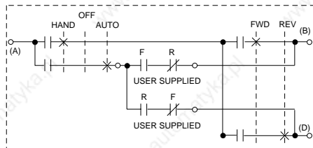
2-WIRE CONTROL W / AUTO START AUTO DIRECTION
