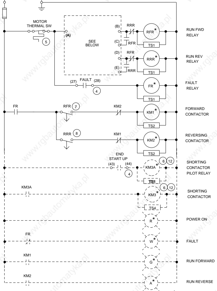
3-WIRE CONTROL
