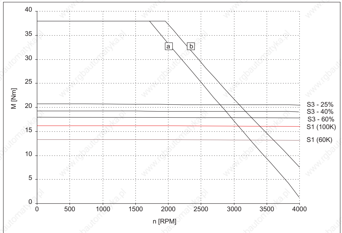
Figure 3-81 Speed-torque diagram 1FT6064-6WF7
