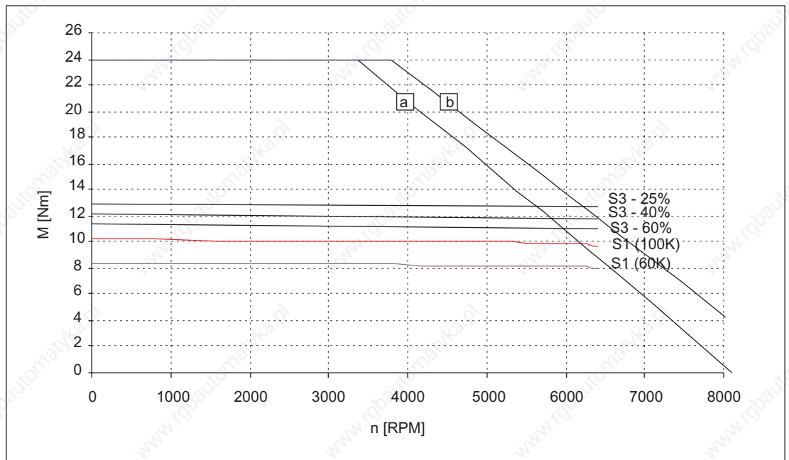
Figure 3-80 Speed-torque diagram 1FT6062-6WK7□
