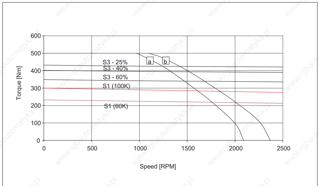
Figure 3-101 Speed-torque diagram 1FT6138-6WB7□
