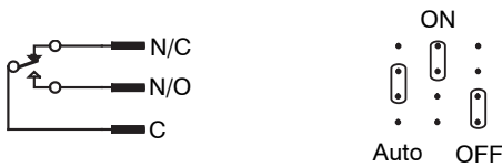
Digital Output (8 identical channels)
