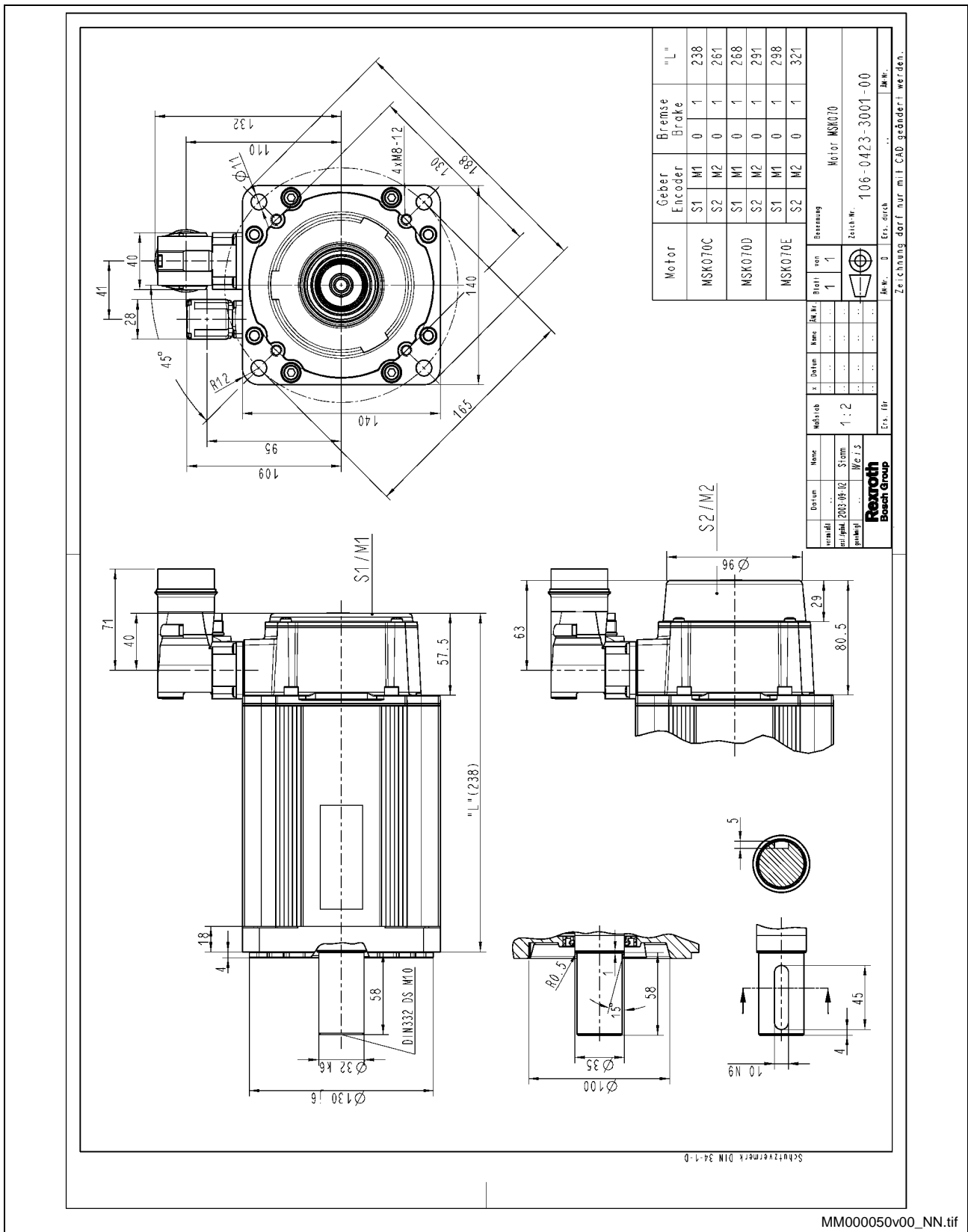
Fig. 5-6: MSK070 specification
