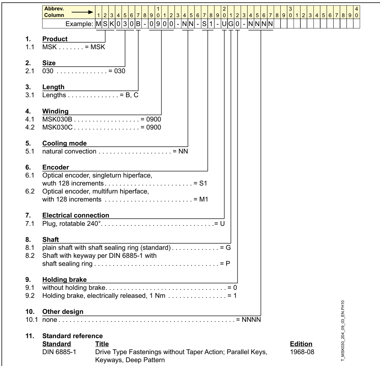
Fig. 6-7: Type code MSK030
