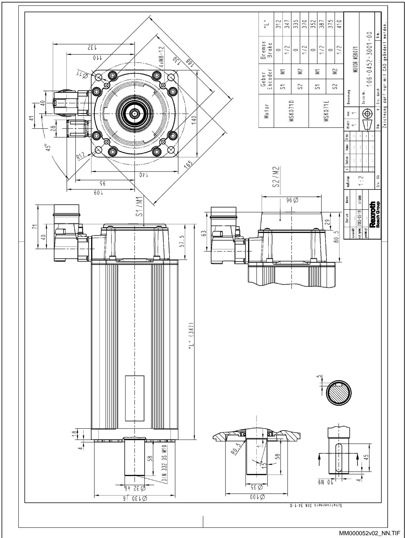
Fig. 5-7: MSK071...NN specification
