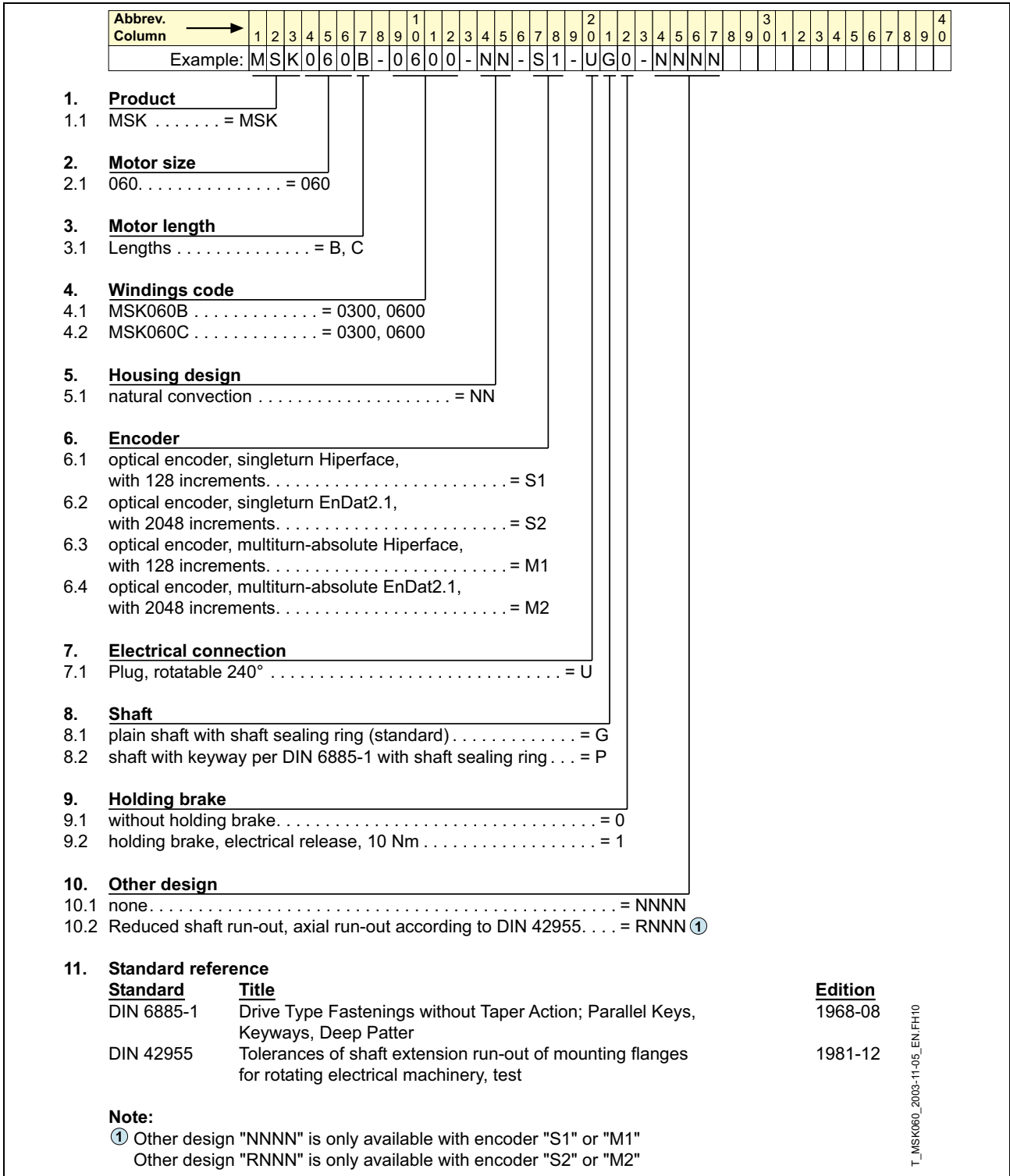
Fig. 6-10: Type code MSK060
