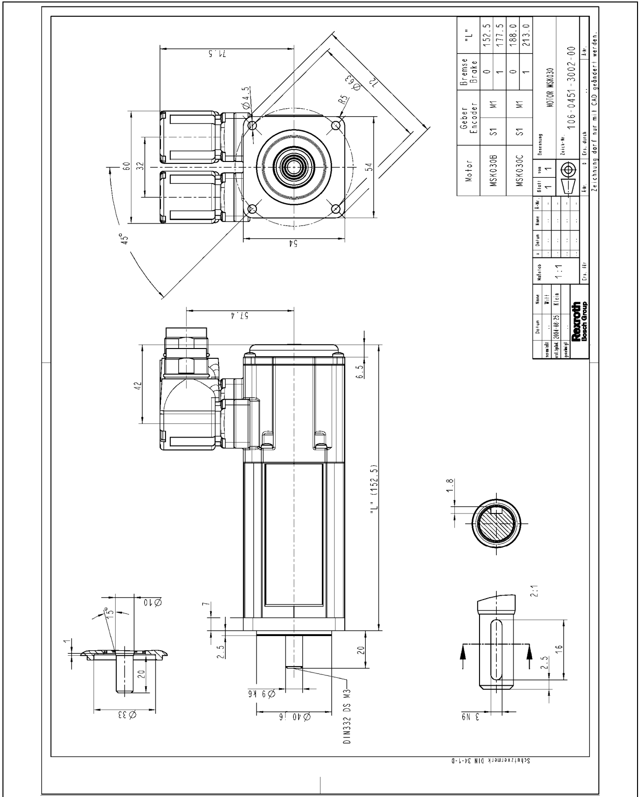
Fig. 5-2: MSK030 specification
