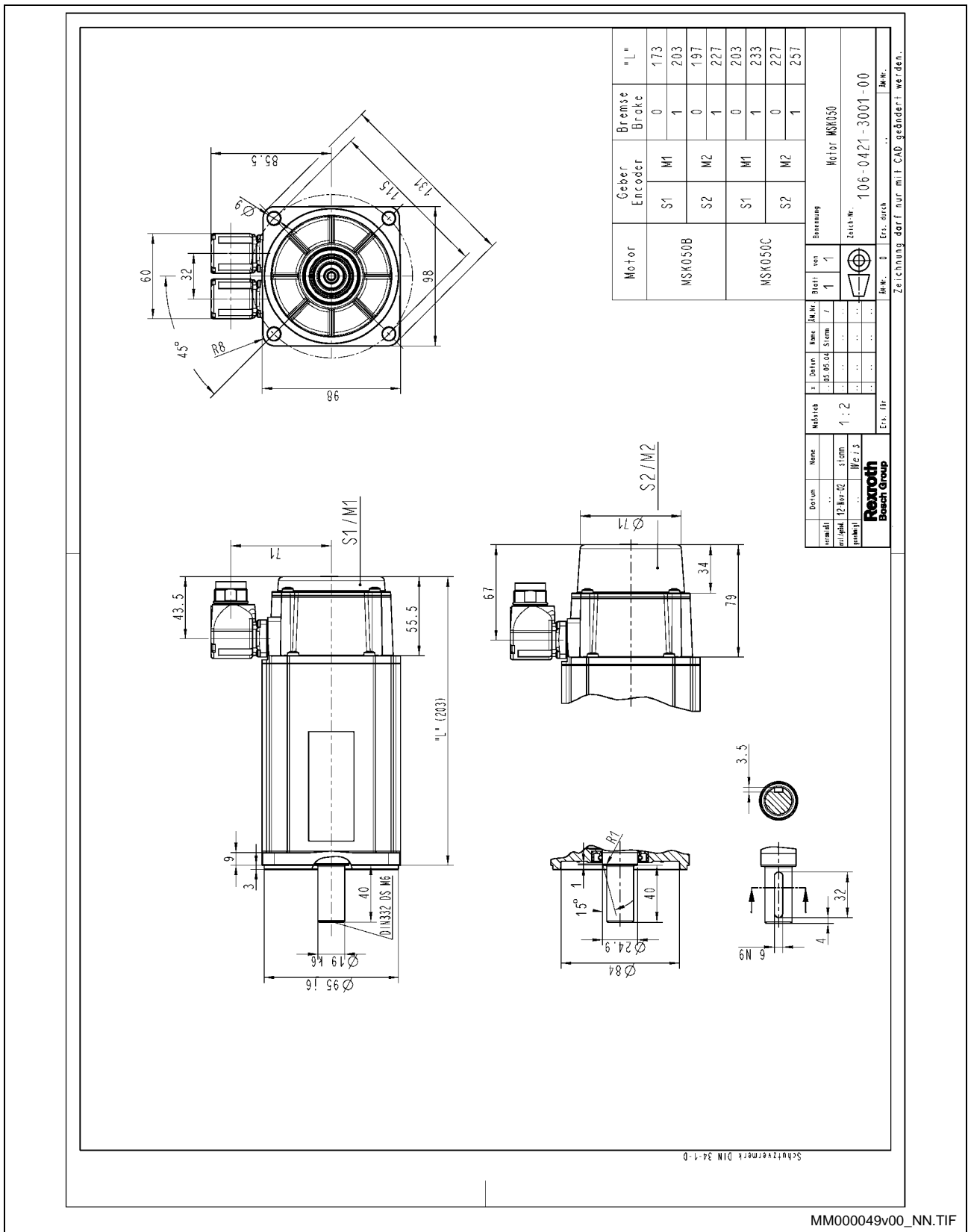
Fig. 5-4: MSK050 specifications
