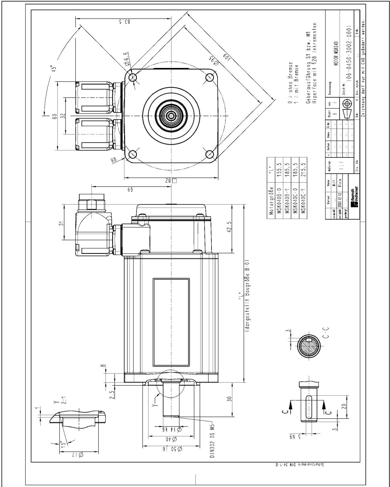
Fig. 5-3: MSK040 specification
