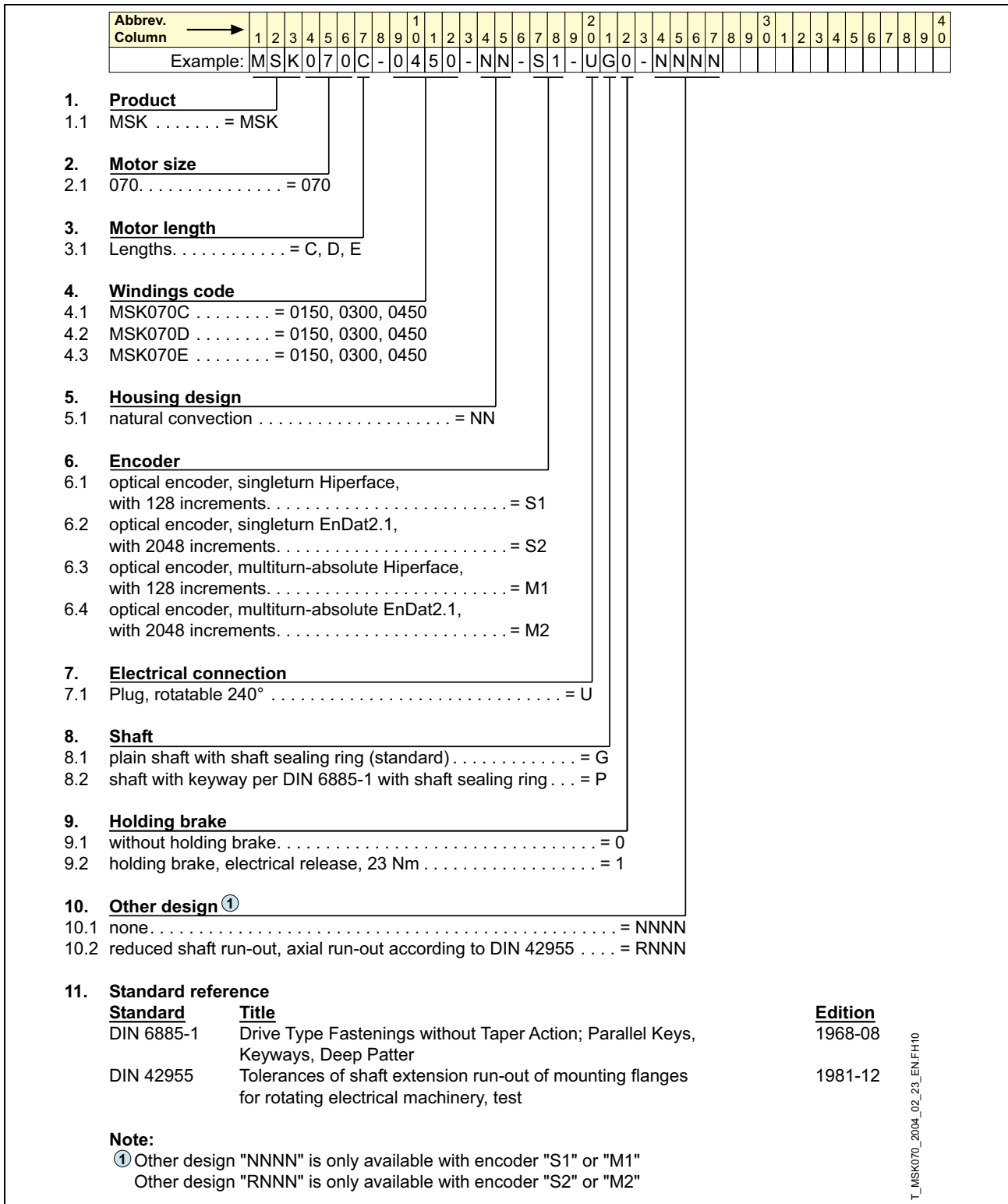
Fig. 6-11: Type code MSK070
