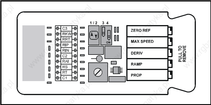
Figure 2-3 Daughter board as supplied by default
