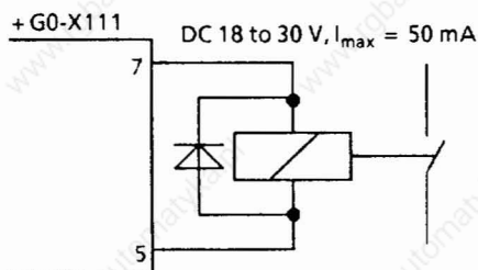
Fig. 3.12 Connection of a relay
