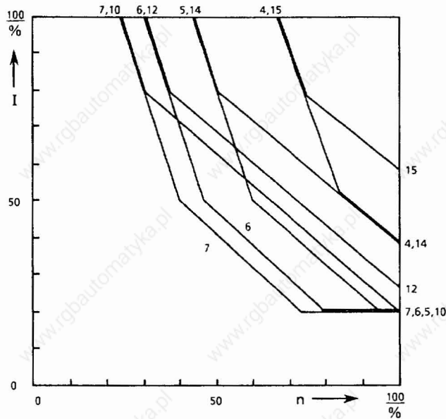
Fig. 3.1 Adjustable characteristics of speed-dependent current limitation
