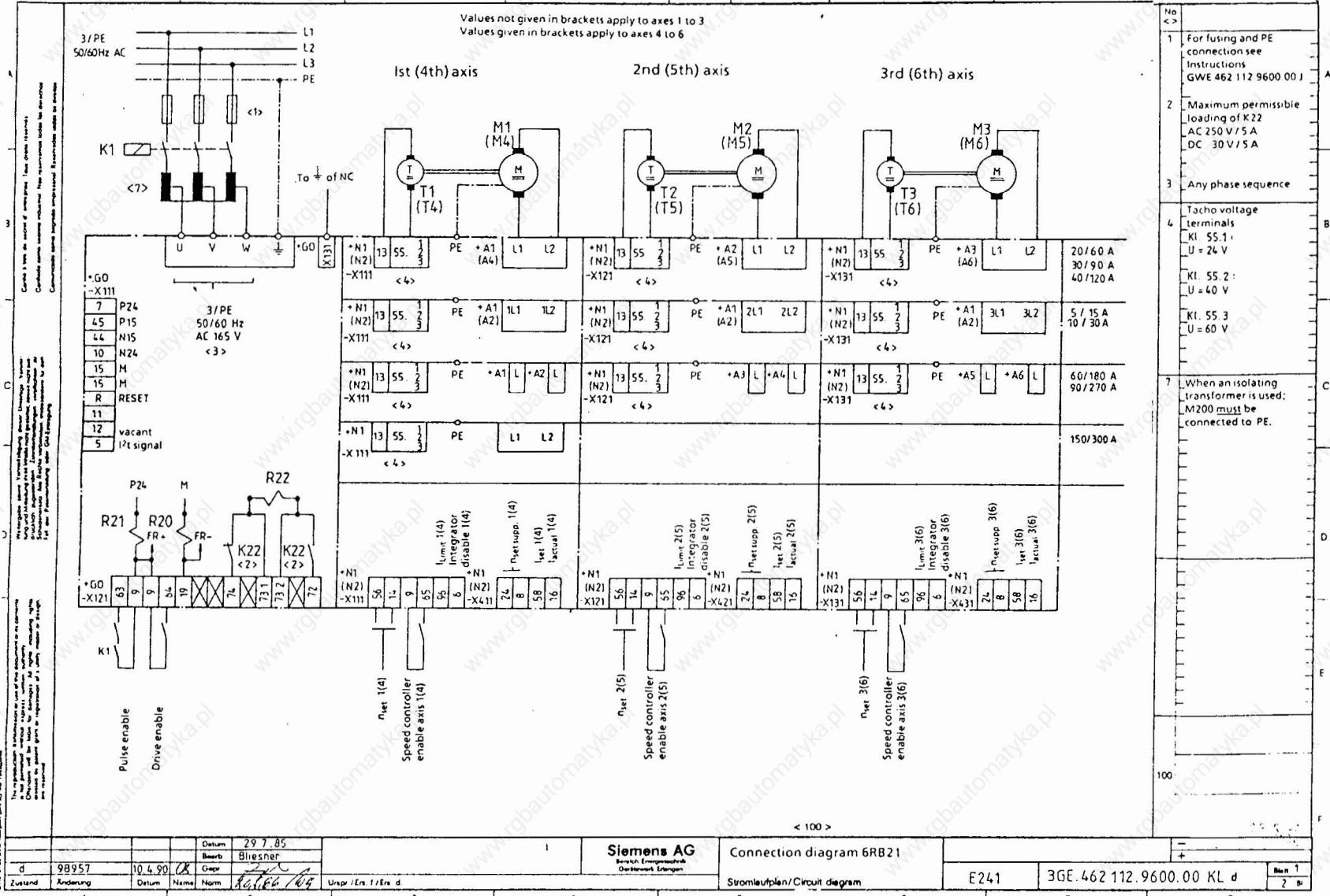
6 Terminal connection diagram
