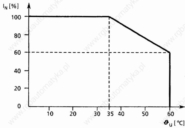
Fig. 1.4 Power reduction with raised inlet air temperature
