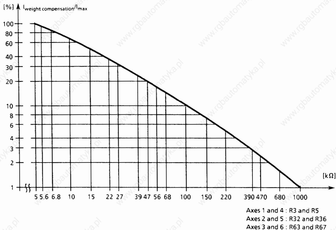
Fig. 3.6 Supplementary current setpoint for electrical weight compensation
