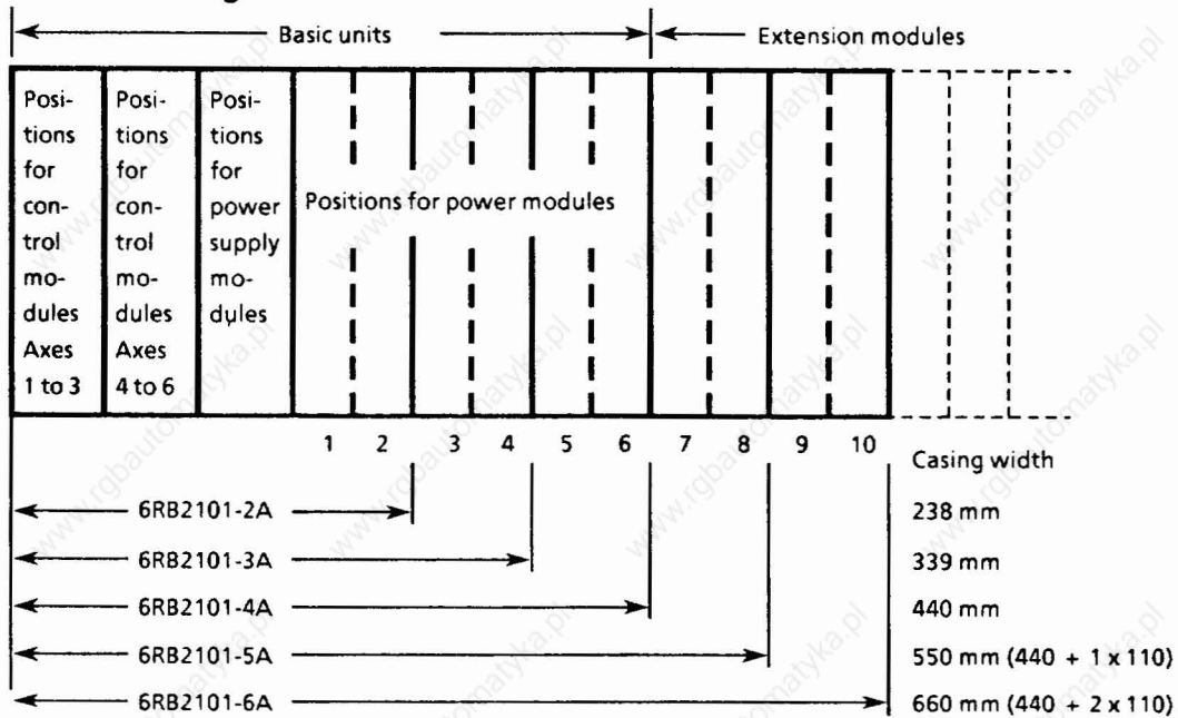
Fig. 1.2 Casing
