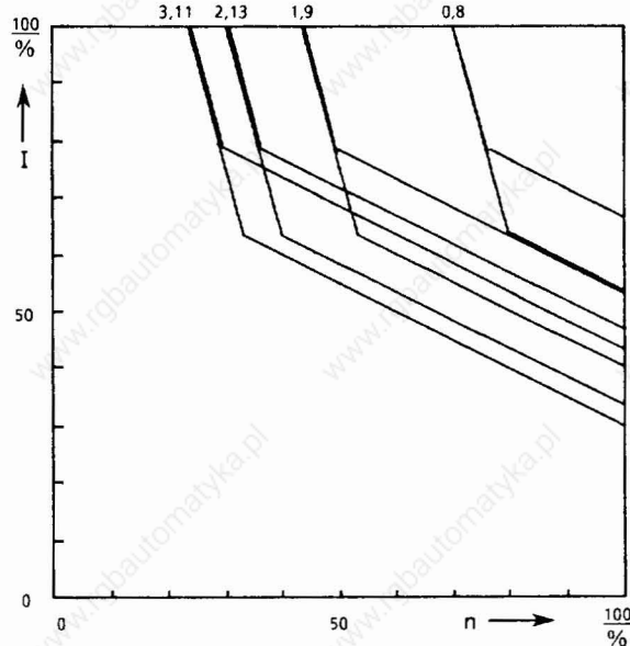
Fig. 3.2 Adjustable characteristics of speed-dependent current limitation
