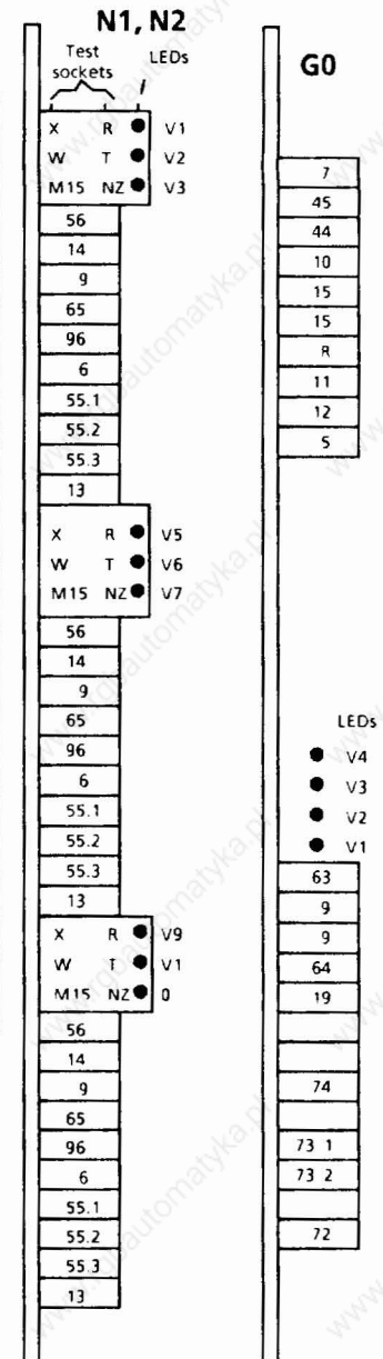
Modules for slots N1, N2 and G0
