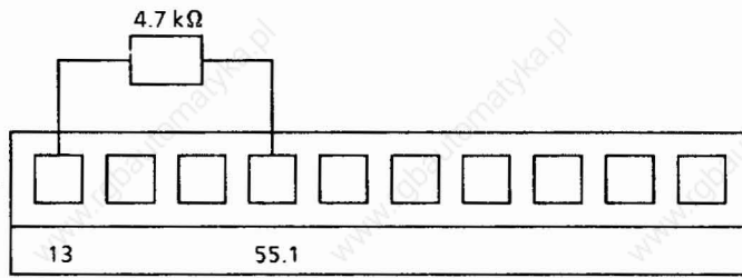
Fig. 3.10 Connector X1.1
