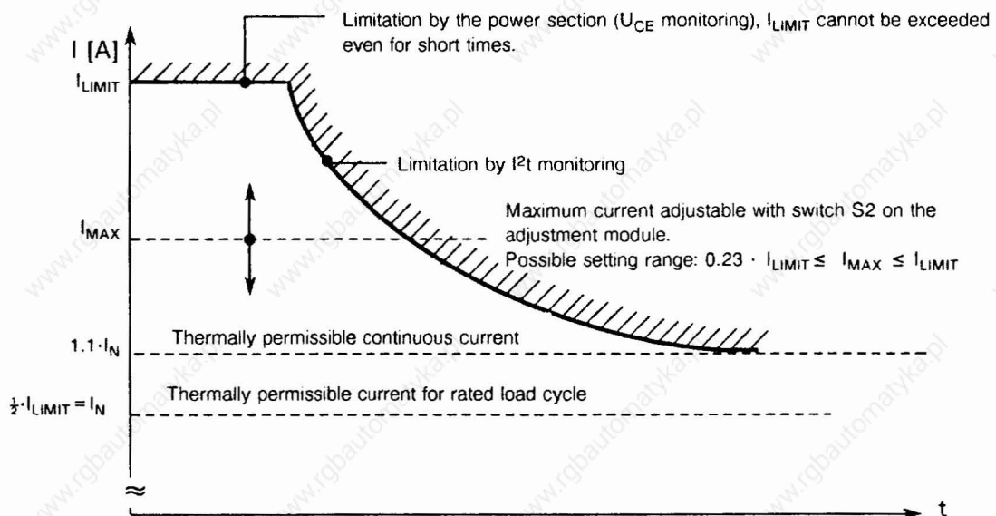
Fig. 1.6 Effective current limits
