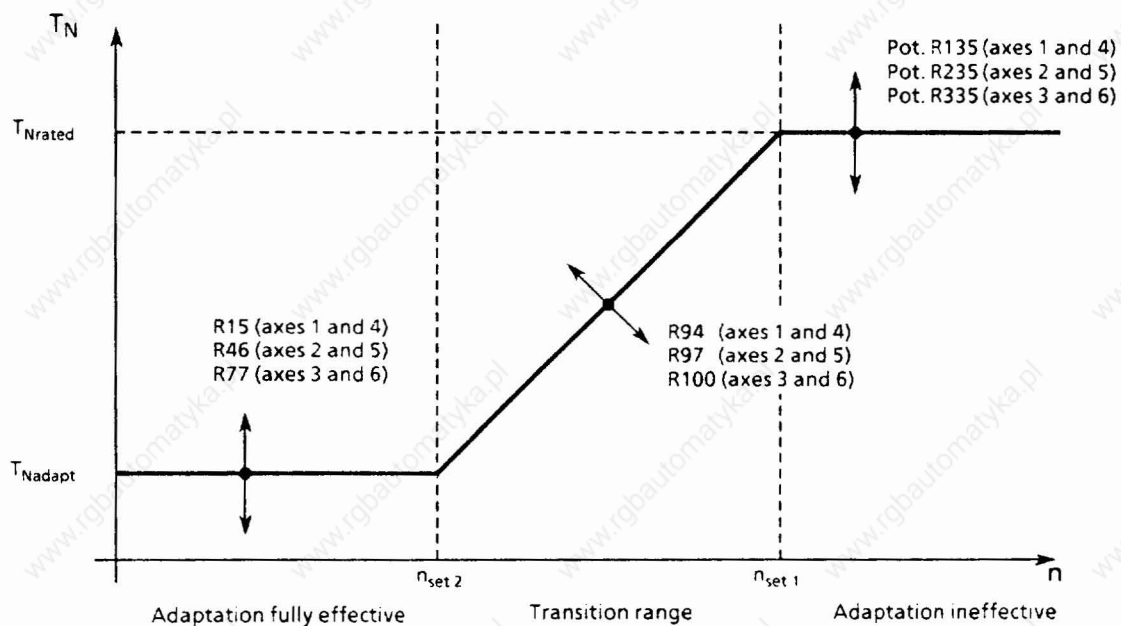
Fig. 3.5 Relationship between reset time and speed
