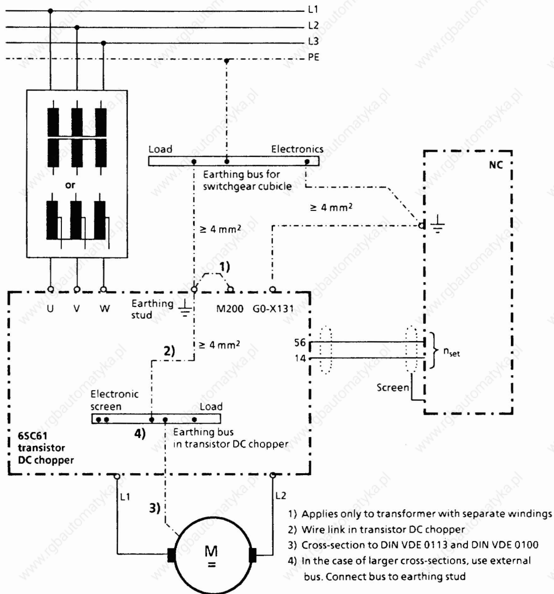
Fig. 2.1 Earthing concept
