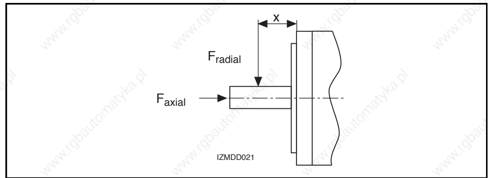
Fig 8.9: Shaft load
