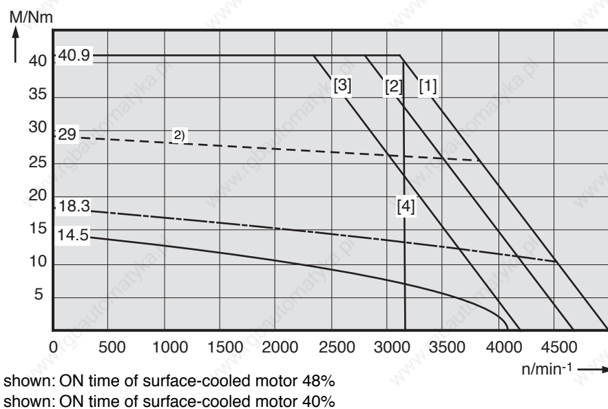
Fig 6.7: Torque-speed characteristics MAC 093
