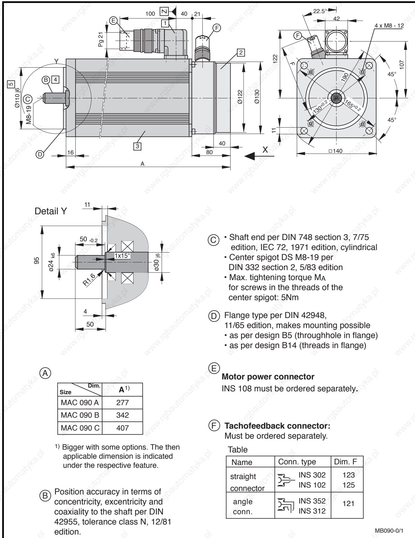
Fig 5.10: Dimensional data - MAC 090 (natural convection)
