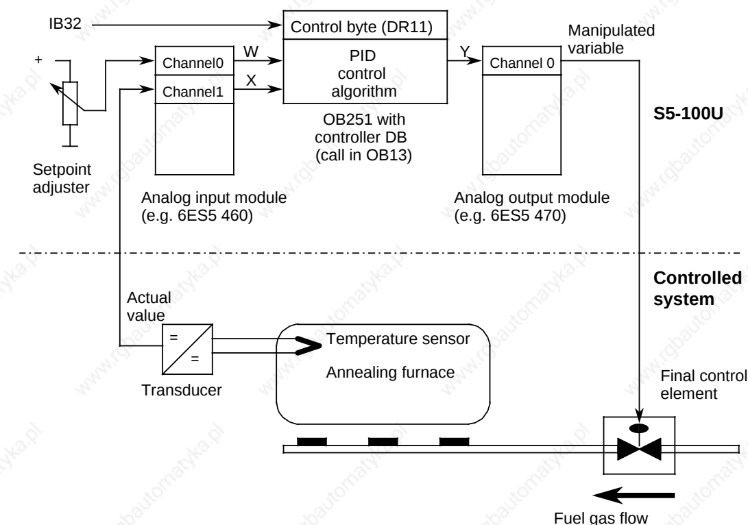
Figure 9-9. Process Schematic
