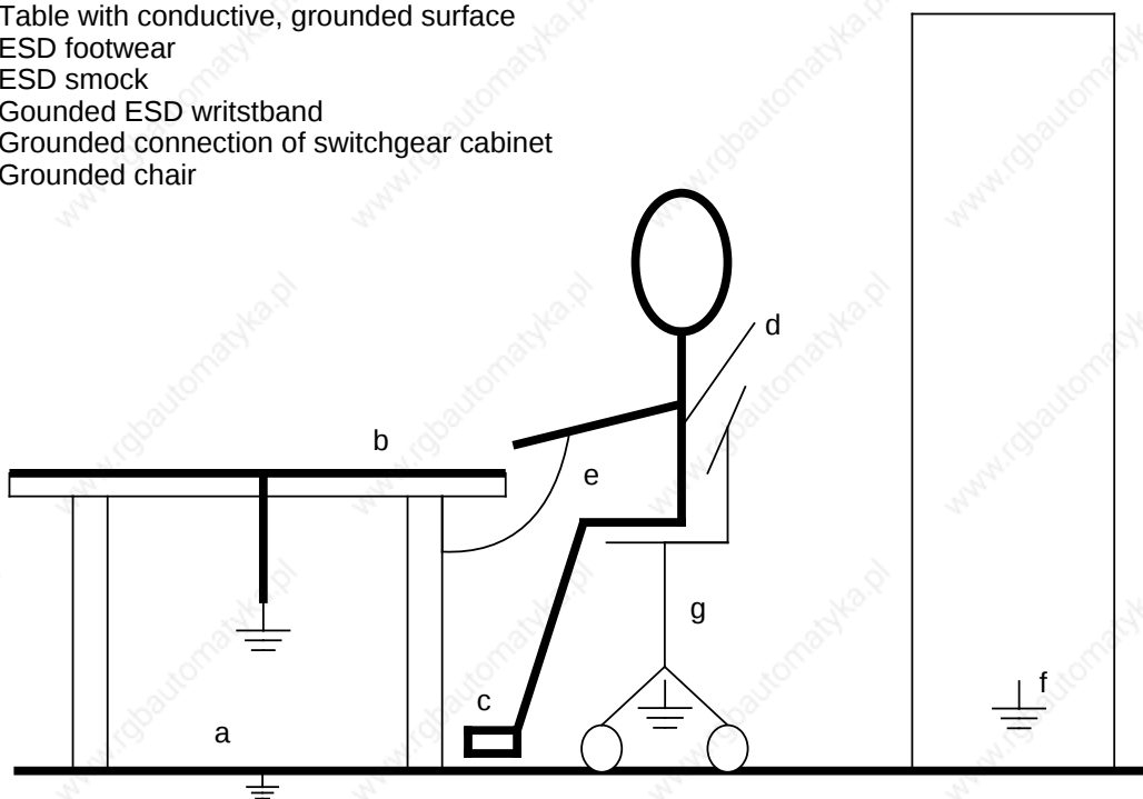
Figure C-1. ESD Measures
