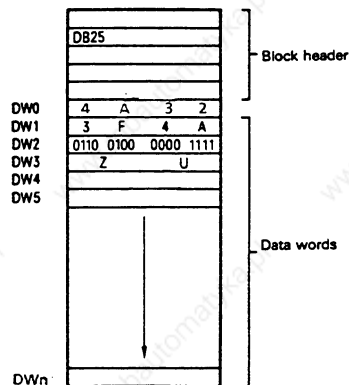
Fig. 7 Structure of a data block
