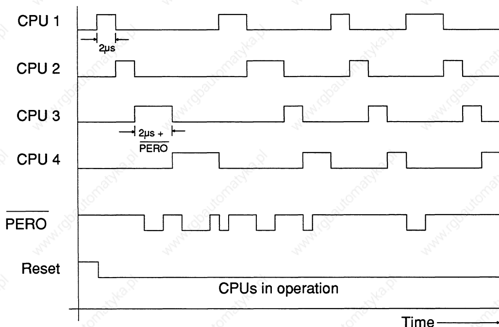
Fig. 1 Operational sequences of the bus control signals
